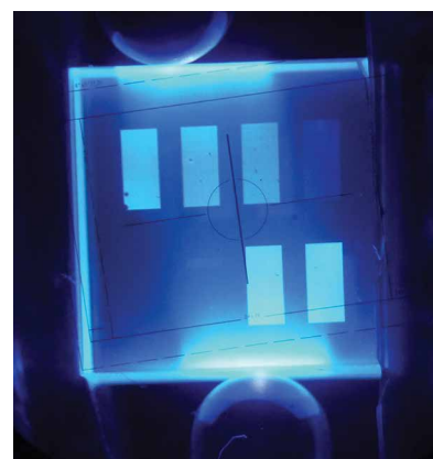
Enhanced scintillation light extraction from a UV-excited LSO crystal, on which six different photonic crystal patterns have been produced
