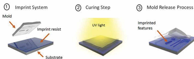
Schematic of the nanoimprinting process used for fabricating the photonic crystals
