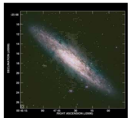
Multiwavelength view and the magnetic field structure of the galaxy NGC253 (provided by V. Heesen)
