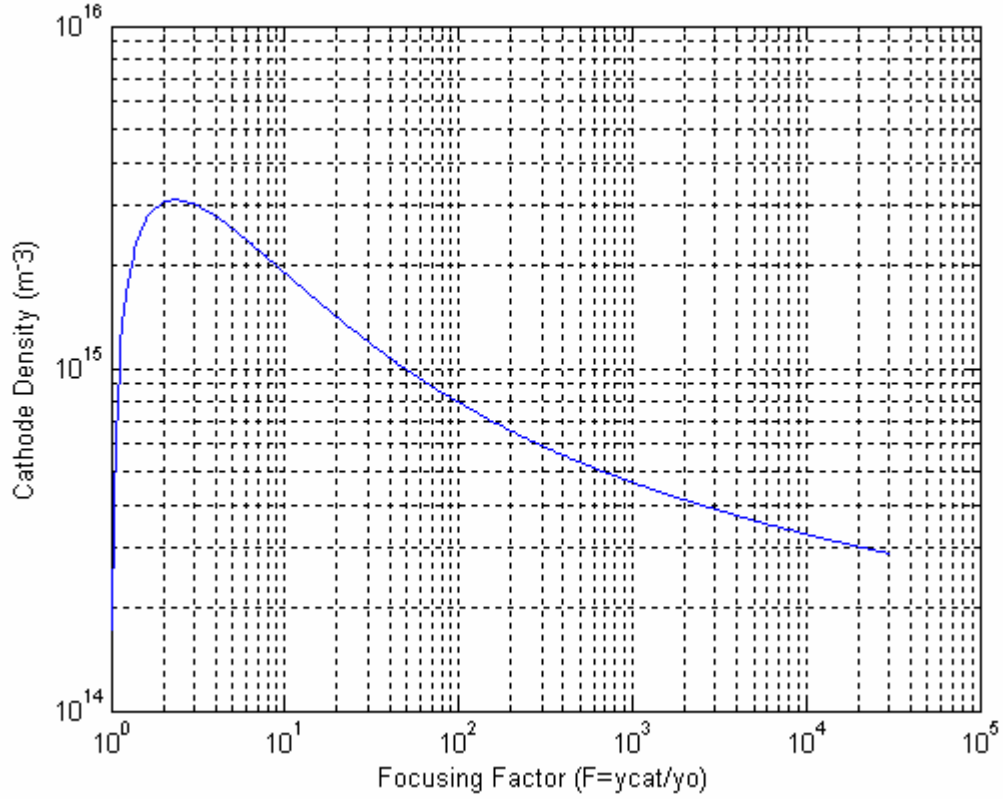
Figure 3.5 Cathode density for 100 keV beams as a function of focusing factor
