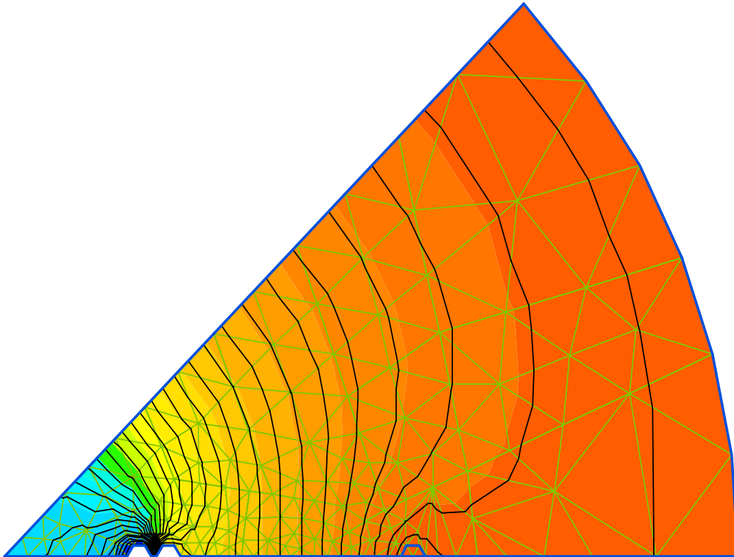
Figure 3.14 Grid triangles and potential solution for 2D FEM wedge model of three grids
