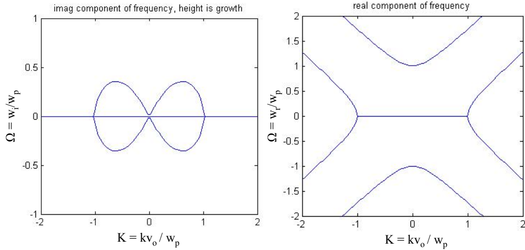
Figure 4.23 2-Stream dispersion relation, imaginary (left) and real (right) solutions, \omega = \omega_r + i\omega_i
