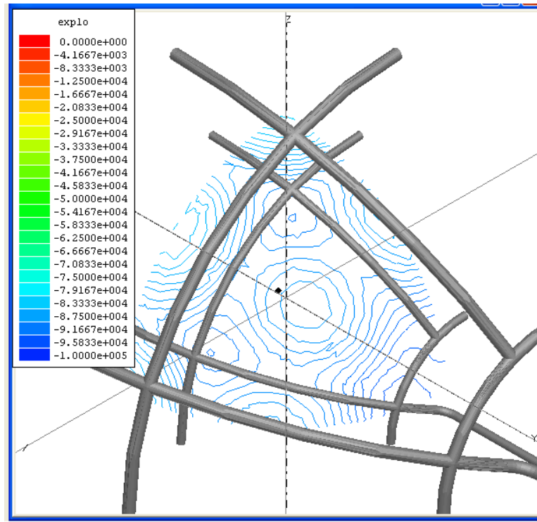
Figure 3.23 Electric potential inside cathode grid for 3D FEM model
