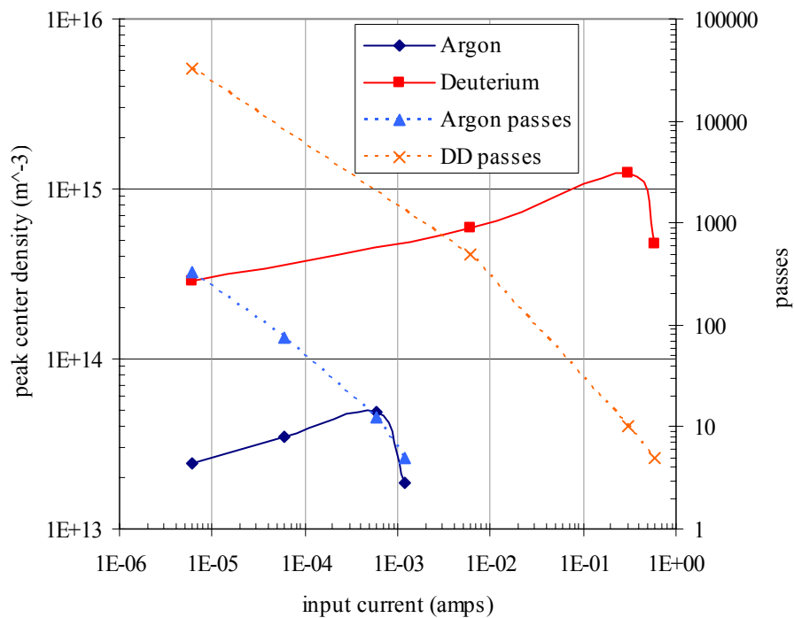
Figure 3.38 Steady-state center peak density in \text{m}^{-3} and confinement time in passes versus input current in amps for Argon and Deuterium
