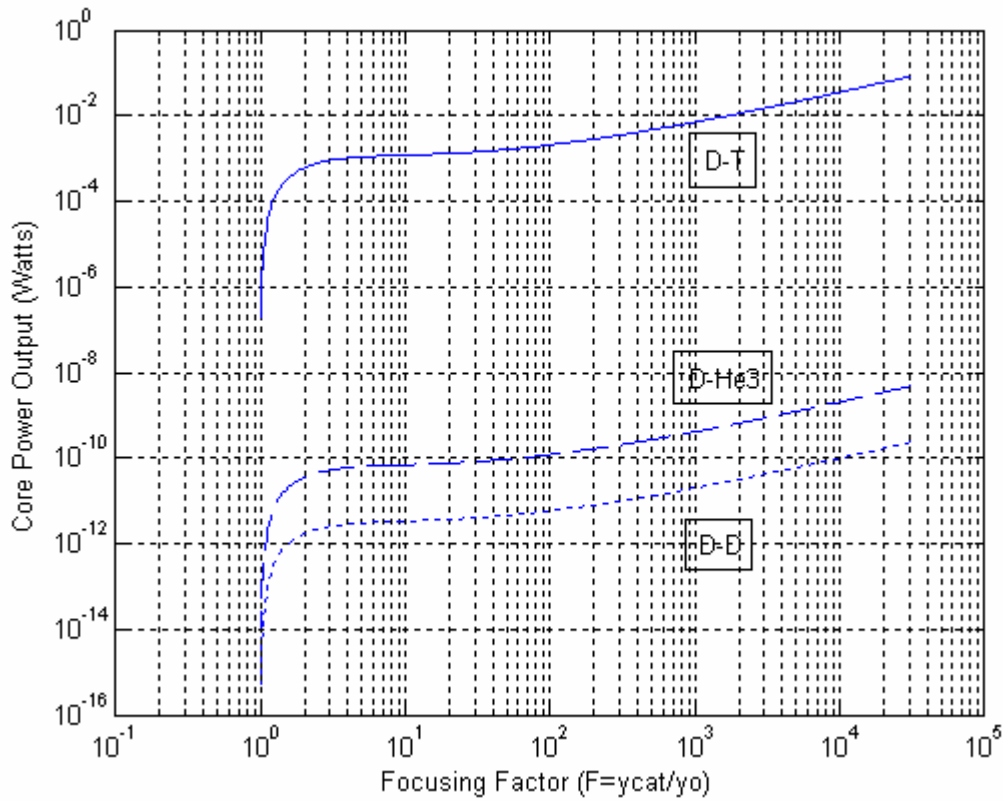
Figure 3.6 Core fusion power for 100 keV beams as a function of focusing factor, (D-T, solid line; D-He 3 , dashed line; D-D, dotted line)
