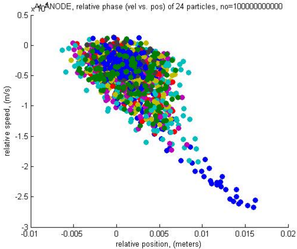
Figure 4.48 Relative speed vs. position for stable synchronization after 100 passes, n_0 = 1 \cdot 10^{11} \text{ m}^{-3} , initial ‘1/10’ spread of 0.018 m.
