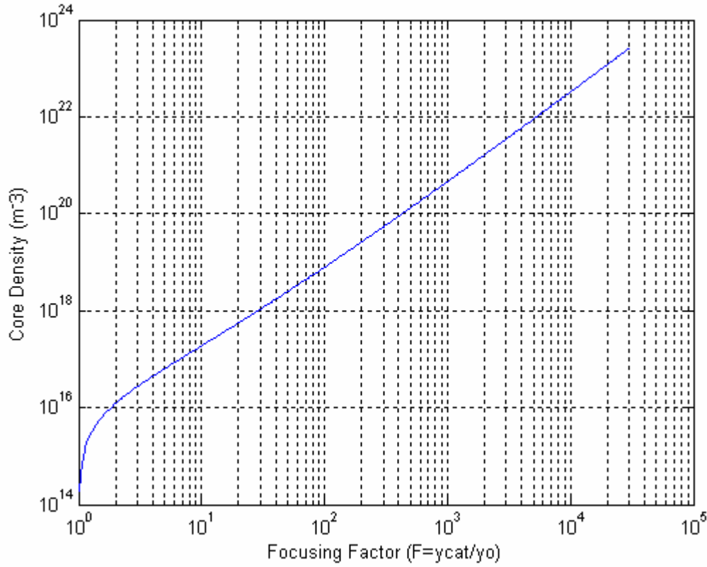
Figure 3.4 Core density for 100 keV beams as a function of focusing factor
