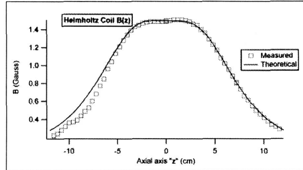
Figure 9. Axial Magnetic Field of Helmholtz Coil
