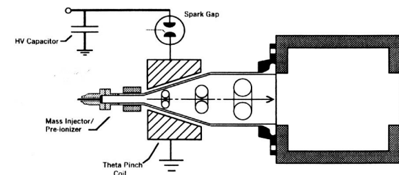
Figure 2. Plasmoid Thruster Experiment (PTX) Schematic
