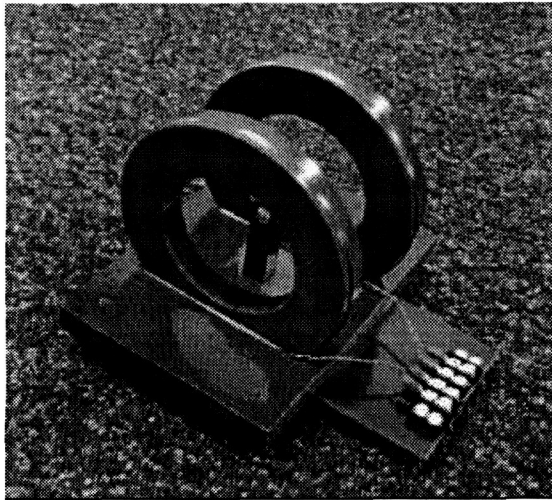
Figure 8. Helmholtz Coil
