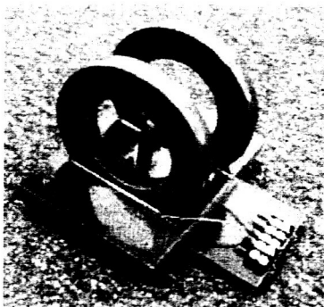
Figure 5. Helmholtz Coil
