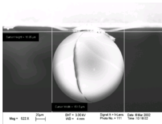
Figure 2.10: SEM image of a gold coated polystyrene sphere with a fracture mounted on an AFM cantilever.
