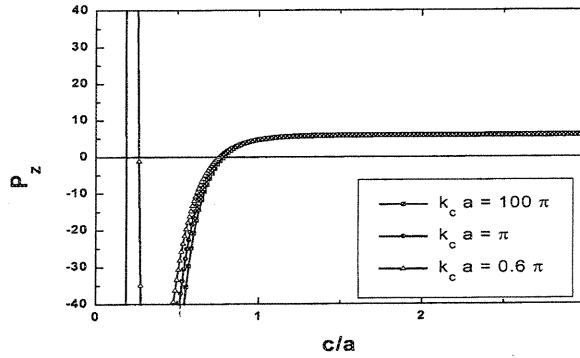
Fig. 4. A magnified view of the pressure P_z (as shown in Figure 2) as a function of c/a for a cavity with a = b , for k_c a = 100\pi, \pi , and 0.6\pi . The pressure is repulsive for c/a > 0.8 independent of different values of the plasma frequency cutoff.
