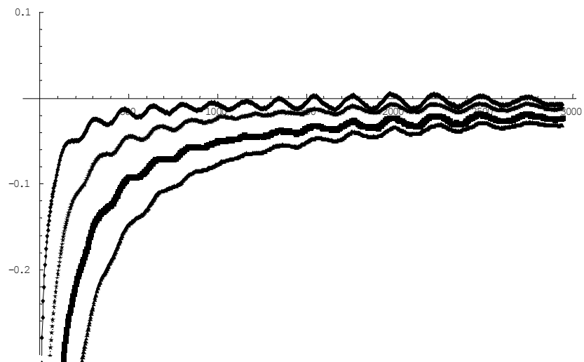
Figure 2.17: AFM photodiode signal versus separation for the data shown in the previous figure, plotted for low values of the photodiode signal.
