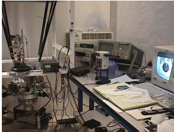
Figure 2.3: The vacuum chamber for the AFM is on the far left. The black shock cords supporting the chamber from the top of the white metal frame are visible. To the right are the electronics, including the monitor showing an image of a cantilever sphere from the CCD camera inside the vacuum chamber.
