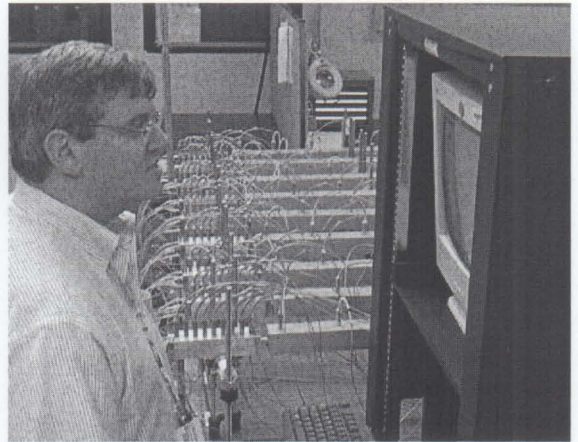
Figure 2. Titanium/water heat pipe test.
