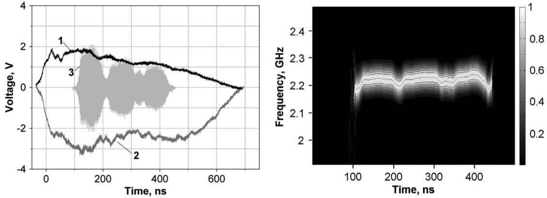
Fig. 5. Left: Accelerating voltage (1, 200 kV/div.), diode current measured by the RC (2, 5 kA/div.), and RF voltage from the B-dot probe (3). Right: Time variation of the radiation spectrum (the RF voltage Fourier transform within the 30-ns time window being shifted by a 1-ns time step). Cathode of [16], d_{AK} = 19 mm, cavity geometry of [16].
