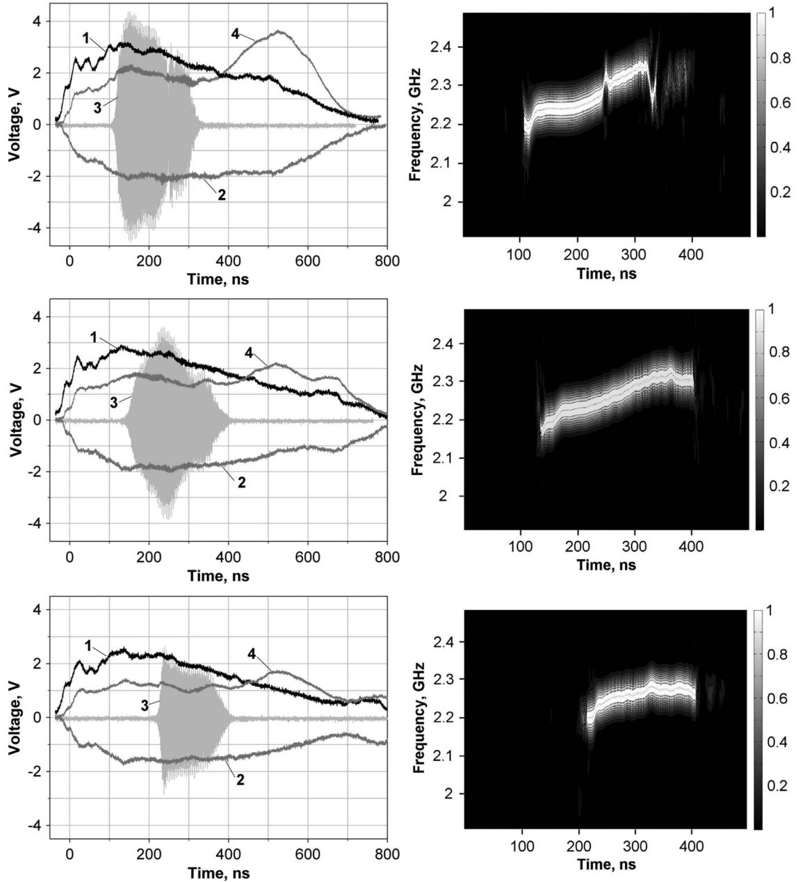
Fig. 9. Left: Accelerating voltage (1, 200 kV/div.), diode current (2, 5 kA/div.), RF voltage from the B-dot probe (3), and current traversing the cavity (4, 1 kA/div.). Right: Time variation of the radiation spectrum. Shots with the cavity geometry of [16] for d_{AK} = 20 mm and different charging voltages U_{ch} of the generator primary storage. From top to bottom, U_{ch} = 37, 34 , and 30 kV.
