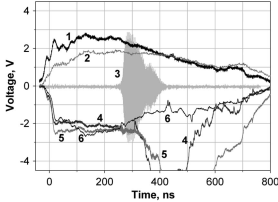
Fig. 11. Accelerating voltage (1, 200 kV/div.), diode current (2, 5 kA/div.), and RF voltage (3) along with the signals from the collimated FCs placed 1 cm behind the vircator cavity at: 4–5 mm off axis; 5–17 mm off axis; 6–30 mm off axis. d_{AK} = 20 mm, U_{ch} = 32 kV.
