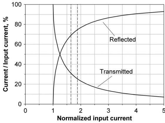
Fig. 13. Percentage of reflected and transmitted currents with respect to the input current according to the 1-D stationary theory for the electron flow with the VC in the equipotential gap. The input current is normalized to I_{cr}^{(1)} . Dashed lines indicate the ratios I_{cr}^{(2)}/I_{cr}^{(1)} for 1 MeV (left) and 100 keV (right) kinetic energy of injected electrons.
