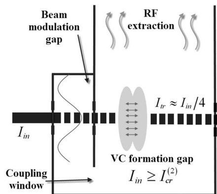
Fig. 1. Schematic of the double-gap vircator interaction space.
