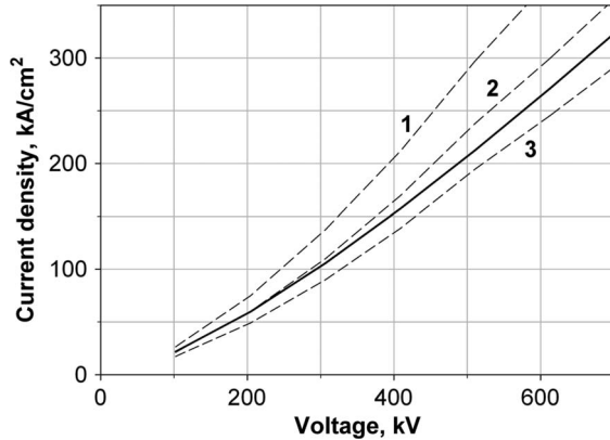
Fig. 2. Solid curve—second critical current density for the planar 5-cm gap calculated according to [13]. Dashed curves—relativistic Child-Langmuir current density for planar diodes with AK gaps of: 1–17 mm; 2–19 mm; 3–21 mm.
