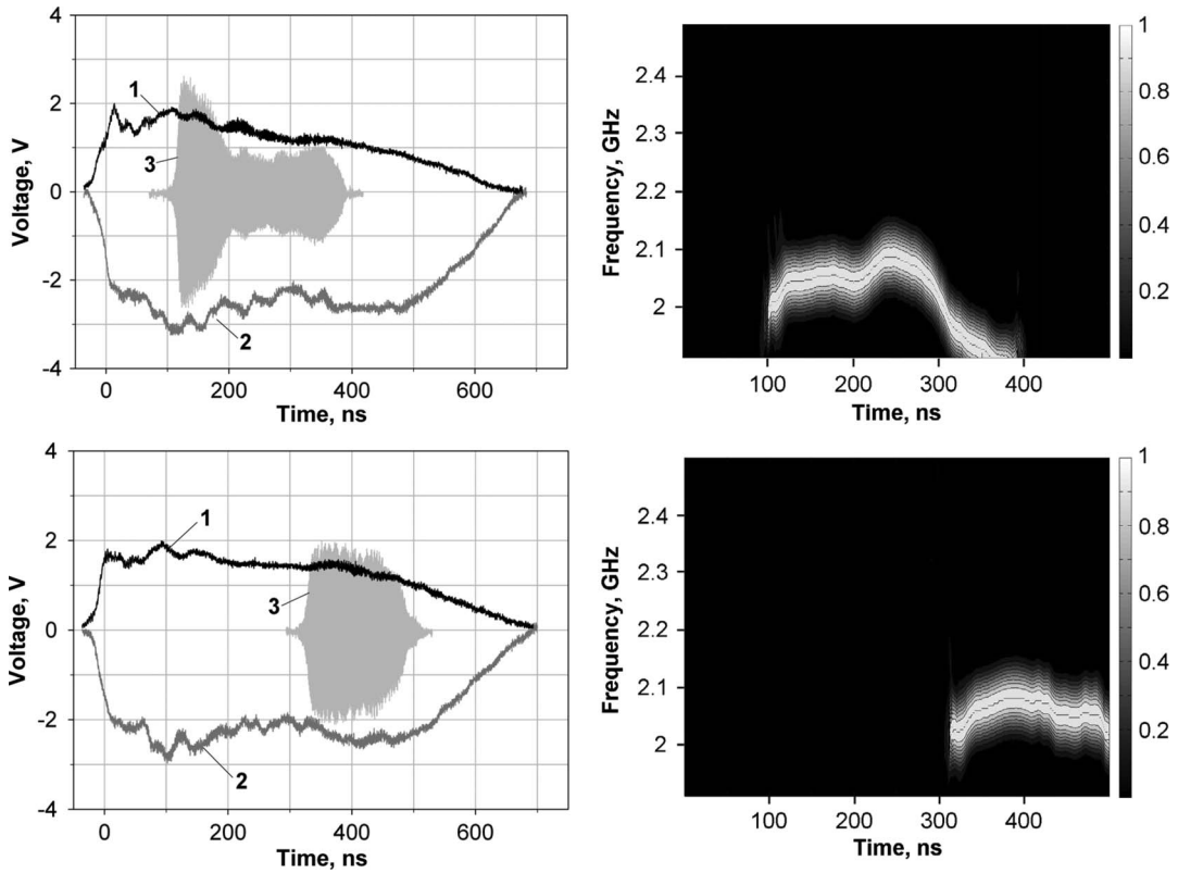
Fig. 6. Shots with the cathode of [16] at the modified geometry of the cavity providing a lower operation frequency. Top: d_{AK} = 19 mm. Bottom: d_{AK} = 22 mm. Left: Accelerating voltage (1, 200 kV/div.), diode current (2, 5 kA/div.), and RF voltage from the B-dot probe (3). Right: Time variation of the radiation spectrum.
