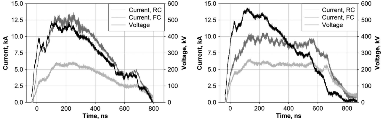
Fig. 7. Pulses of the diode voltage, total diode current, and current delivered to the FC behind the grid anode of the planar diode with the cathode of [16] (left) and improved cathode (right). d_{AK} = 20 mm.
