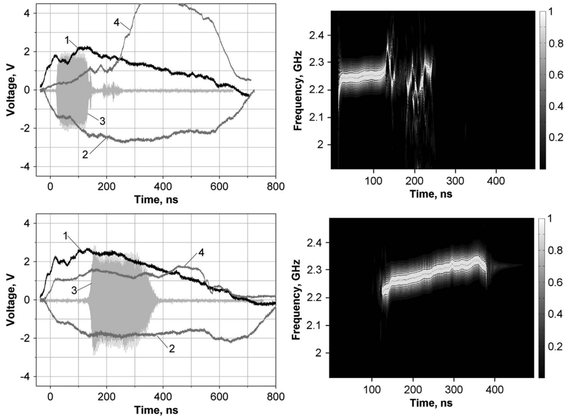
Fig. 10. Left: Accelerating voltage (1, 200 kV/div.), diode current (2, 5 kA/div.), RF voltage from the B-dot probe (3), and current traversing the cavity (4, 1 kA/div.). Right: Time variation of the radiation spectrum. Shots with the cavity geometry of [16] for U_{ch} = 33 kV at d_{AK} = 15 mm (top) and d_{AK} = 19 mm (bottom).
