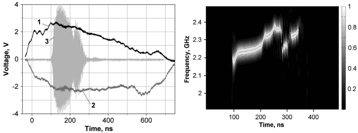
Fig. 8. Left: Accelerating voltage (1, 200 kV/div.), diode current (2, 5 kA/div.), and RF voltage from the B-dot probe (3). Right: Time variation of the radiation spectrum. Improved velvet cathode, d_{AK} = 19 mm, cavity geometry of [16].
