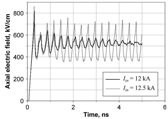
Fig. 14. Axial electric field versus time for different injected currents. The observation point is on the axis, 0.5 cm from the foil in the second section of the cavity. The kinetic energy of injected electrons is 500 keV.
