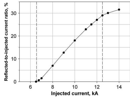
Fig. 15. Percentage of reflected electrons (the difference between the injected current and the current delivered to the cavity back and lateral surfaces averaged over the simulation time) versus injected current. Vertical dashed lines indicate the interval of currents corresponding to a quasistationary state with the VC. The kinetic energy of injected electrons is 500 keV.
