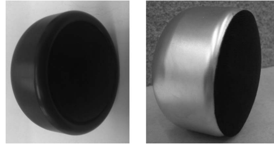
Fig. 4. Left: velvet cathode with the screening electrode coated with ceramics. Right: velvet cathode used in [16].
