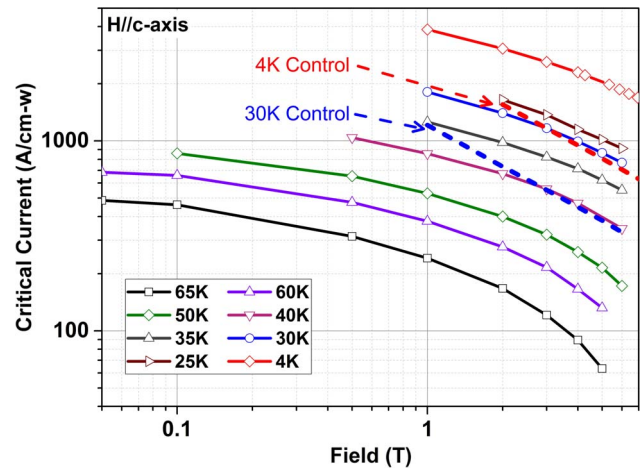
Fig. 7. I_c as a function of temperature and field ( H/c ) for a Au irradiated wire. I_c values for unirradiated control samples at 4 and 30 K (dash lines) are included for comparison.
