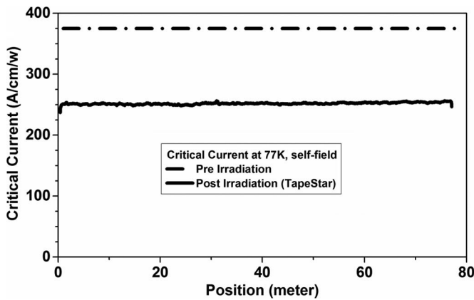
Fig. 6. I_c (77 K, self-field) as a function of length for a coil wire made from a 46-mm strip after irradiation to a dose of 6 \times 10^{11} Au/cm 2 . The preirradiation value is estimated from pieces cut from the ends of the original 46-mm strip.
