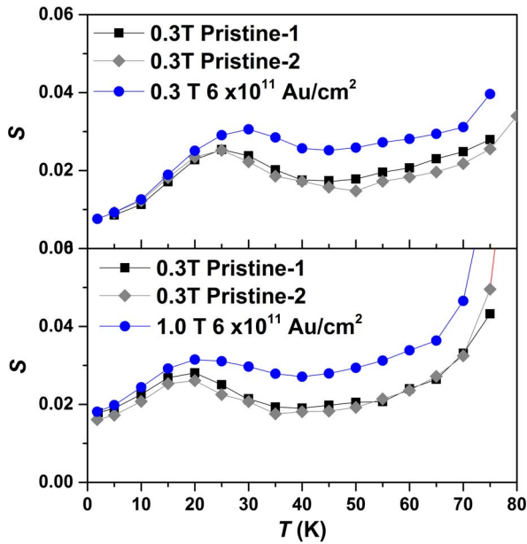
Fig. 3. Flux creep rate as a function of temperature for an Au irradiated sample at 0.3 T (upper figure) and 1.0 T (lower figure). S(T) for unirradiated controls are included for comparison.
