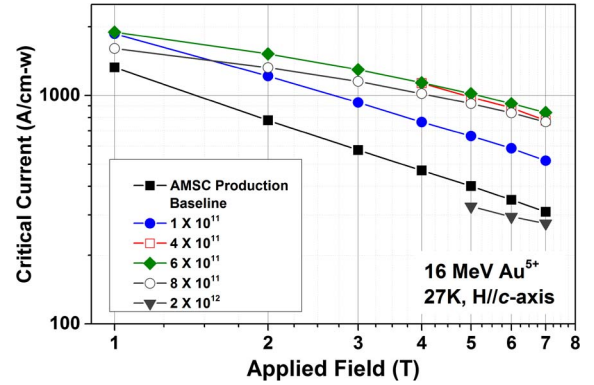
Fig. 1. I_c as a function of magnetic field (H//c) at 27 K for the different doses of Au ions.
