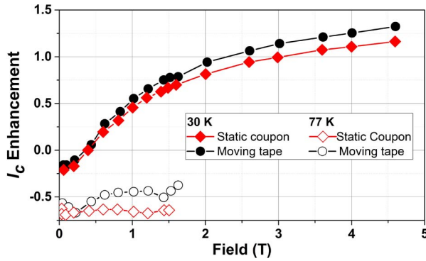
Fig. 2. I_c enhancement at 30 and 77 K (relative to an unirradiated control sample) of a stationary short sample and a moving 1-m tape after irradiation with 18-MeV Au to a dose of 6 \times 10^{11} Au/cm 2 .
