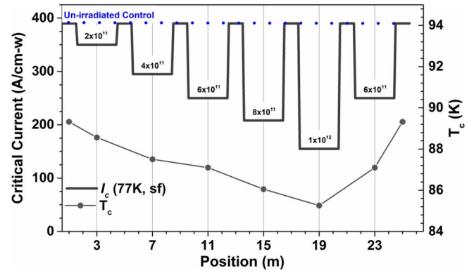
Fig. 4. I_c and T_c along the length of a 10-mm-wide tape as a function of dose of 16-MeV Au ions after irradiation of a moving 46-mm-wide production coated conductor tape. I_c of the unirradiated control sections of the tape are indicated by the dotted line.
