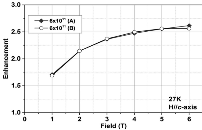
Fig. 5. I_c enhancement measured in two separate 10-mm tapes slit from the 46-mm strip after the roll-to-roll irradiation.
