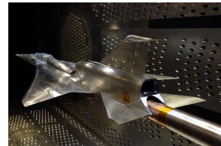
QueSST Aerodynamic Model (aft)
