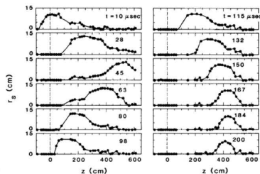
Experimental measurements of excluded magnetic flux for FRC translation
