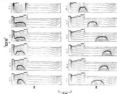
MHD simulation of poloidal flux for FRC translation
