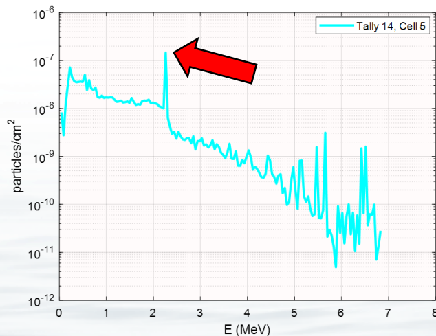
Figure 4. Energy spectrum of gamma flux (#/cm 2 ) into NaI detector, per 2.45 MeV neutron emitted from Pd wire. 45kV resolution.
