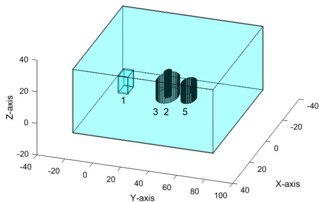
Figure 1. Simulation geometry (cm scale): lucite filled D 2 O chamber (1) with 3 He detector (2) surrounded by HDPE (3) and NaI gamma detector (5).
