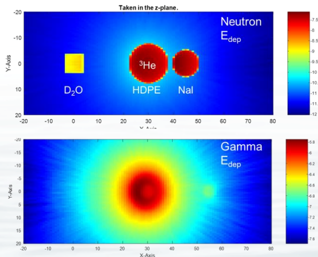
Figure 2. Energy deposited (MeV/g) in materials: (a) Neutron energy deposited in D 2 O and HDPE (C 2 H 4 ) surrounding 3 He detector. Neutrons also reach the NaI behind HDPE; (b) Gamma energy isotropically emitted from HDPE and deposited in NaI detector and D 2 O.
