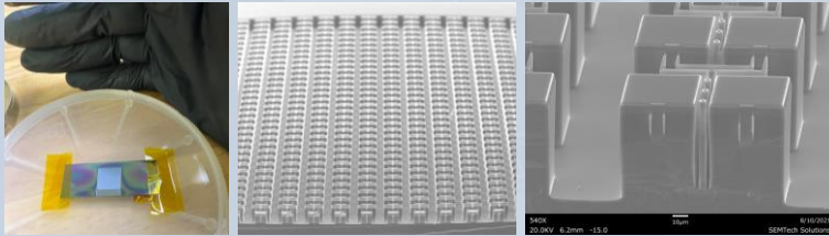
6000 cavity test article
