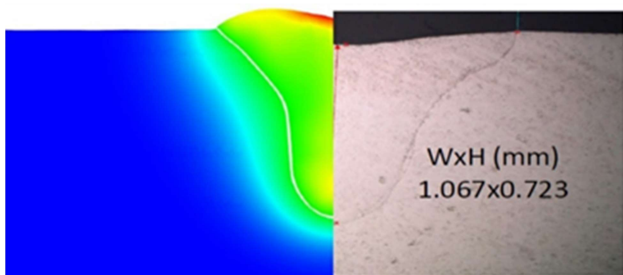
Figure 7. Developing reduced-physics models for quick turn-around analysis of production welds is critically important in numerous stockpile applications. On the left is a melt pool for a stainless-steel weld as predicted by a reduced-physics model calibrated to weld data on the right. This is an example of a challenging multiscale, multiphysics problem that requires fast-running tools for effective production work. (SNL)
