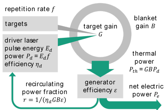
Fig. 18: Basic parameters of an IFE power plant (left). Illustration of a “ 1\ \omega beam box” providing 8.1 kJ at 1.05\ \mu\text{m} (converted to 5.7 kJ at 0.35\ \mu\text{m} close to the target chamber) as a modular component of an IFE laser system (right) [Bay2011].
