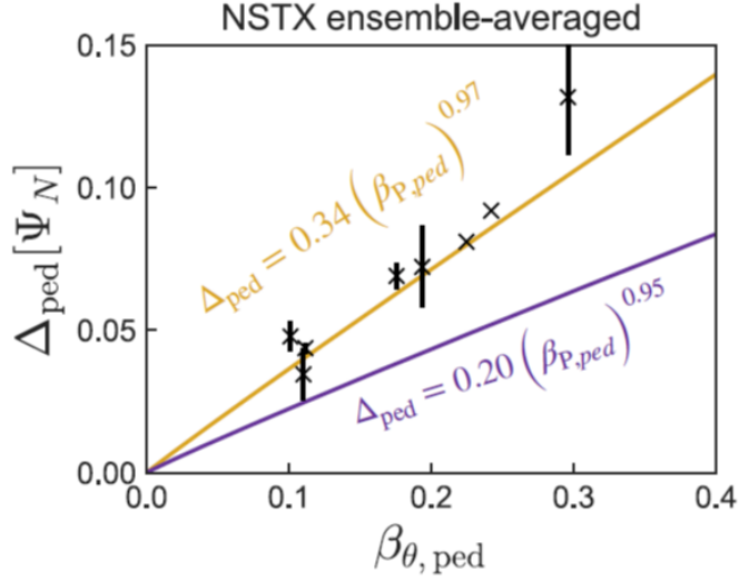
Figure 2. Pedestal width in \Psi_N , \Delta_{\text{ped}} , vs. pedestal height in \beta for various experimental NSTX discharges. The ideal ballooning critical pedestal prediction (purple) falls short of predicting the width, while the new gyrokinetic critical pedestal prediction matches the data.
