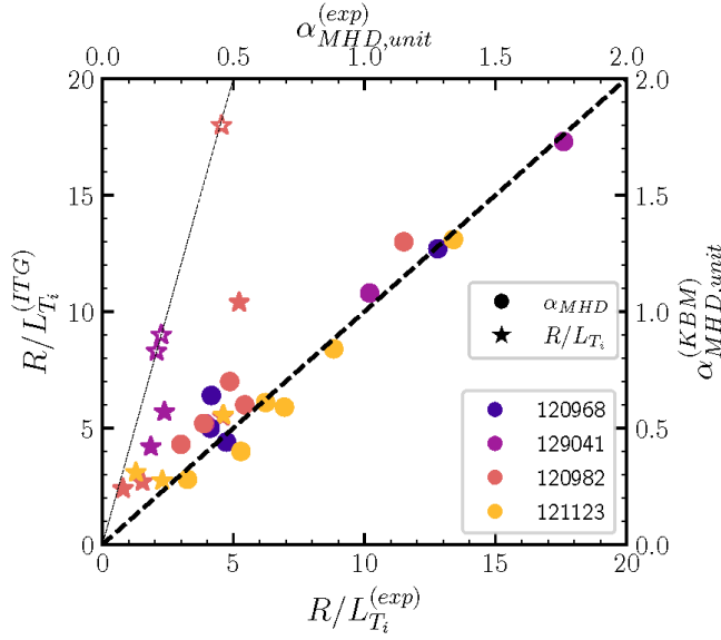
Figure 4. Summary of ITG thresholds ( R/L_{T_i} , on bottom and left axes) and KBM thresholds ( \alpha_{MHD,unit} , on top and right axes) calculated with gyrokinetic (CGYRO) simulations against the corresponding experimental value, combining different discharges and radial positions. The thick dashed line represents the condition where a threshold matches the experimental value.
