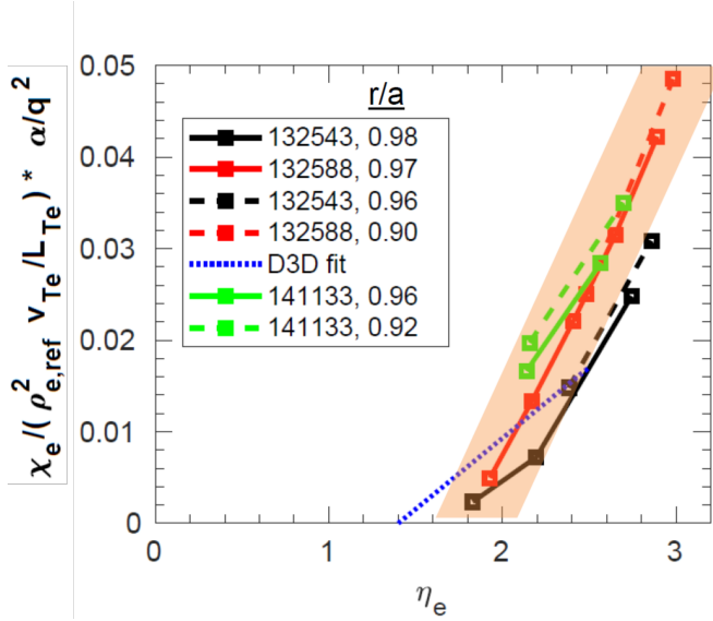
Figure 3. A threshold-based reduced model for ETG transport shows overlap between NSTX and DIII-D simulations when \alpha/q^2 , which goes like local equilibrium pressure gradient, is accounted for in plotting the gyroBohm-scaling-normalized ETG diffusion coefficient vs. the ETG drive, \eta_e , the ratio of density and temperature scale lengths.
