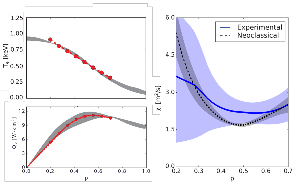
Figure 5. (top left) Predicted electron temperature profile from TGYRO for a NSTX H-mode discharge 129017 at \sim 0.45 s, using input from a TRANSP run (red) compared to the experimental profile (gray). (bottom left) TGYRO prediction compared to the experimentally inferred turbulent electron energy flux. (right) Ion heat diffusivity which follows neoclassical.
