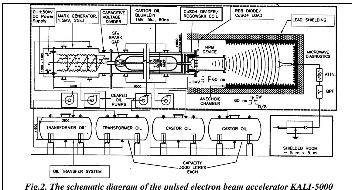
The schematic of this pulsed electron beam accelerator is presented in Fig.2. It comprised of high voltage \pm 50 kV DC charging power supply followed by an impulse generator based on plus minus charging type Marx generator. The output pulse is shaped
