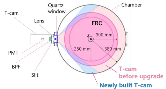
Figure 2. Comparison of the field of view, newly built T-cam and before upgrade.
