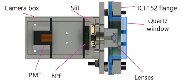
Figure 1. The incident optics is placed inside of the window (cross-section view).
