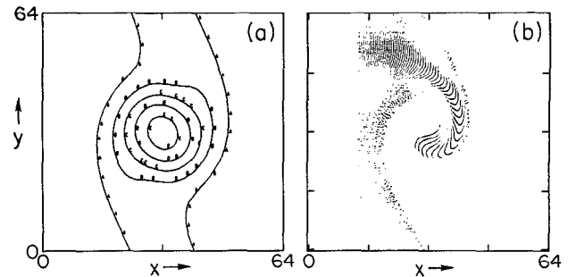
FIG. 4. (a) Contour plot of the electrostatic potential at the critical time shown in (b). (b) Position of particles in the (x-y) plane with initial fluid velocities v_y < 0 at a critical stage of dynamics just before wave breaking.
