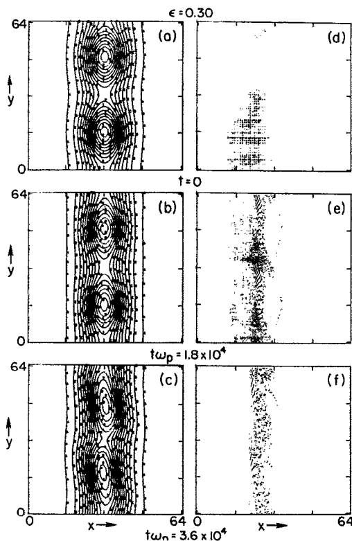
FIG. 11. Potential contours (a)–(c) and particle plots (d)–(f) for the period-doubling coalescence of the m = 2 , \epsilon = 0.30 island chain. The skewness of each vortex as the axis between two vortex centers rotates during coalescence.
