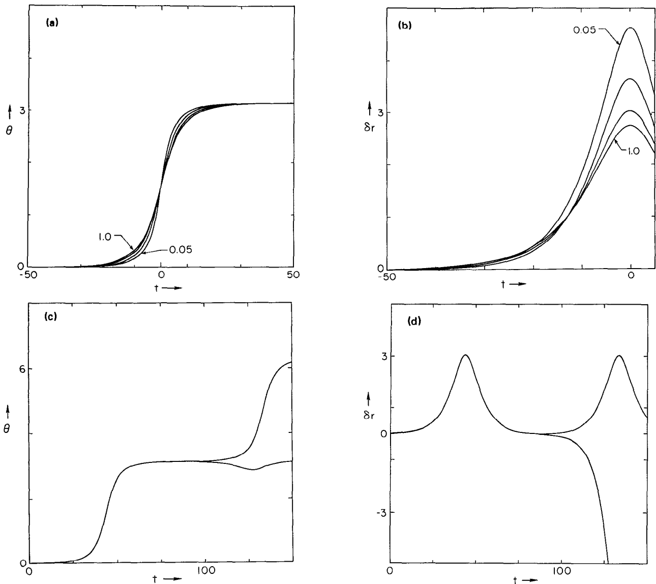
FIG. 18. Nonlinear results of the localized vortex model. (a) \theta(t) for \varepsilon = 0.05, 0.30, 0.70 , and 1.0 . (b) \delta r(t) for the same \varepsilon values. (c) Plots of \theta(t) that show trajectories with initial conditions on the two sides of the separatrix. (d) \delta r(t) for two initial conditions, one just inside and the other just outside the separatrix.
