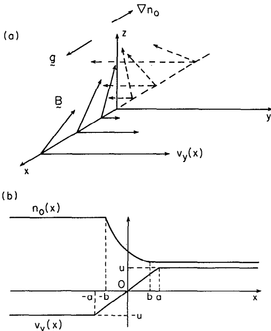
FIG. 1. (a) Slab geometry showing coordinates used to describe the sheared magnetic field \mathbf{B}(x) and sheared flow velocity \mathbf{v}_y(x) along with the directions of \nabla n_0 and \mathbf{g} . (b) The piecewise continuous profiles of the sheared flow velocity v_y(x) and the density n_0(x) .
