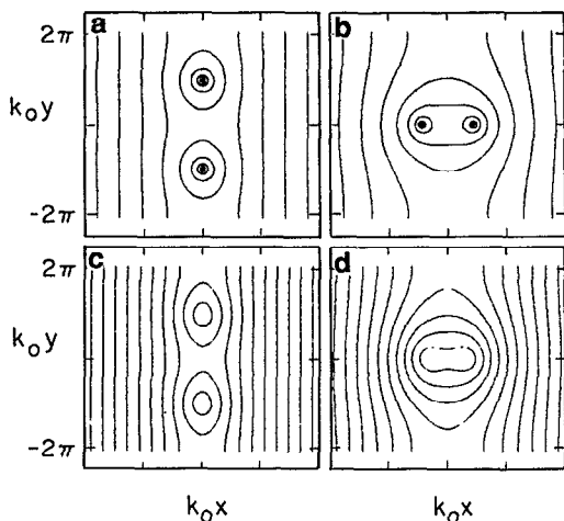
FIG. 19. The streamfunction for the cases: (a) \phi(x, y, 0; 1) , (b) \phi(x, y, \hat{t}; 1) , (c) \phi(x, y, 0; 0.6) , and (d) \phi(x, y, \bar{t}; 0.6) . Here \hat{t} and \bar{t} are chosen so that the rotation is approximately 180^\circ .
