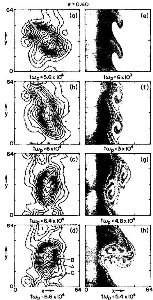
FIG. 12. As in Fig. 11, but a case of \epsilon = 0.6 with stronger tilting, where the rotation continues after coalescence.
