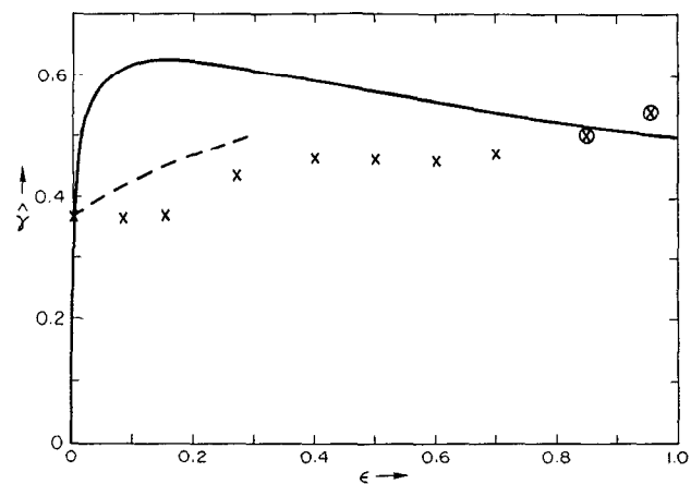
FIG. 9. Plot of normalized linear growth rate \hat{\gamma} vs \epsilon : \times represents a data point extracted from the simulation results, \otimes is a data point where it is difficult to ascertain the growth rate because the growth is faster than exponential. The dashed curve is the linear theory of Ref. 25; the solid curve is that derived from the localized vortex model.
