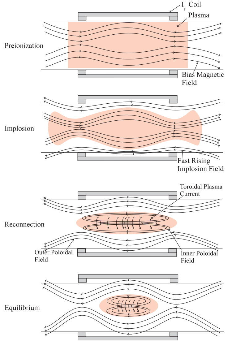
Figure 2: Schematics illustrating the FRC formation process.
