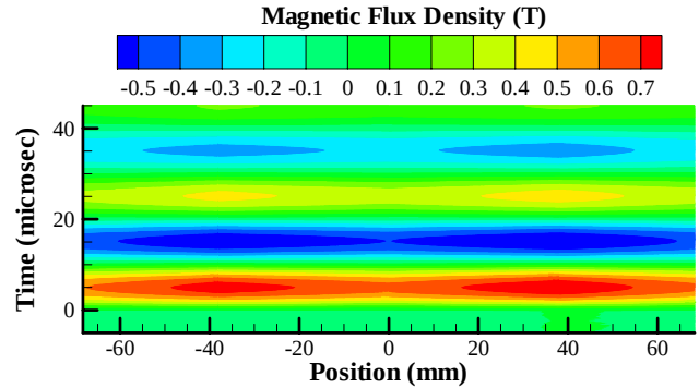
Figure 12: Experimental measurements of the time evolution of the magnetic field.
