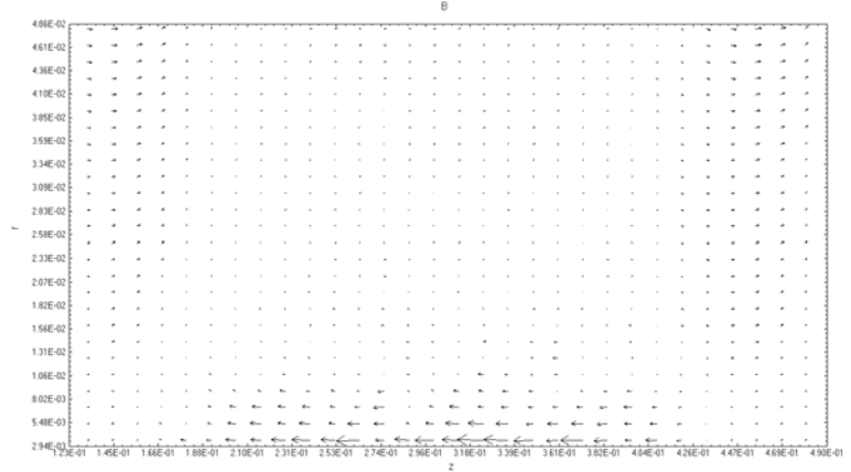
Figure 4: Magnetic field vector in r-z plane showing a small FRC resulting from the conventional helicon model.
