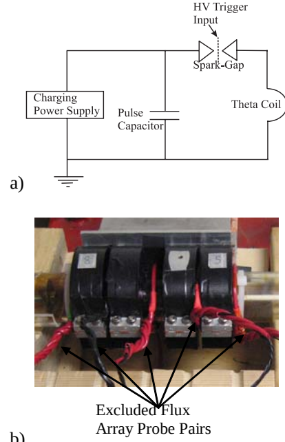
Figure 10: a) Schematic of the PFN and b) photograph of the theta coil with excluded flux array probe pairs.
