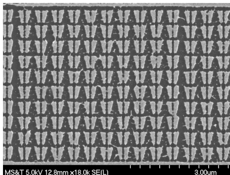
Figure 7: Subsection of the 50x50 Nano-unit Array Used for Optical Characterization
