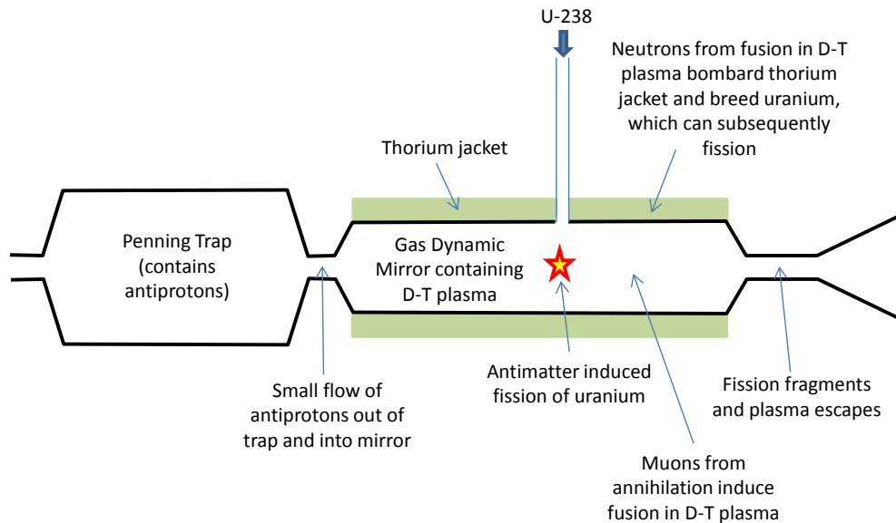
Figure 9 – Antimatter-Induced Fission-Fusion Concept with Thorium Jacket
