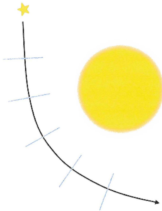
Figure 2. Light-Bending in a Spacetime-Altered Region
