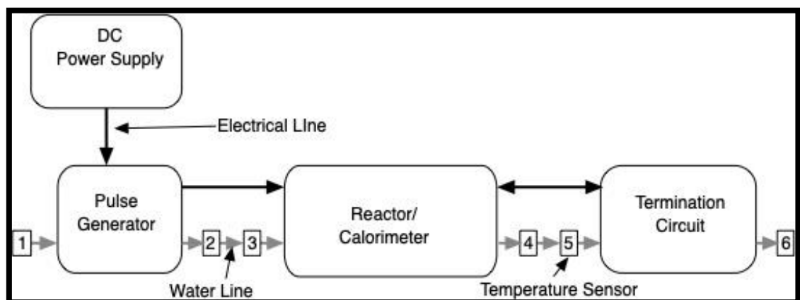
Figure 1. Diagram of mass flow water and pulse stimulation lines.
