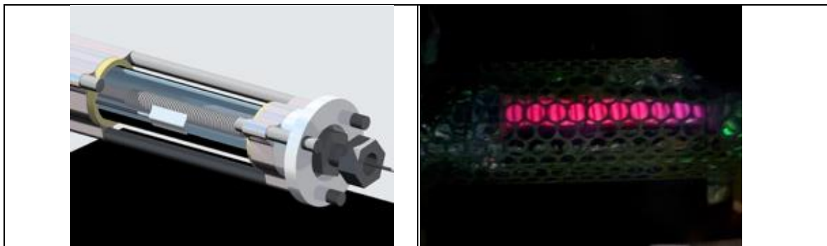
Left: schematic of the reactor design. Right: photograph of the reactor core viewed through the glass outer wall, showing the characteristic red glow of an argon-deuterium plasma, using a new geometric assembly.
