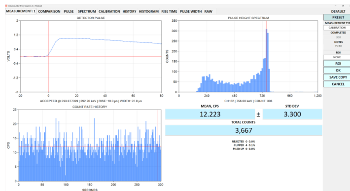
Fig. 3. PulseCounter Pro software thermal neutron spectrum.
