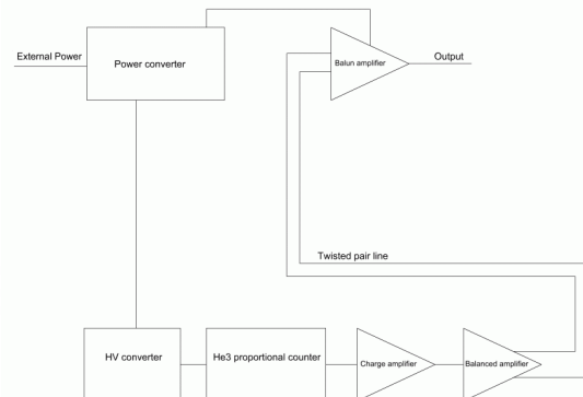
Fig. 2. NEUTRON-X block diagram.
