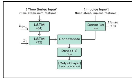
Fig. 1 Block diagram of neural network
