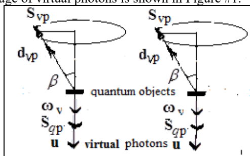
Figure #1. The schematic image of virtual photons created by positively charged quantum objects with parallel spins ( S_{qp} ) constituting orthohydrogen.
