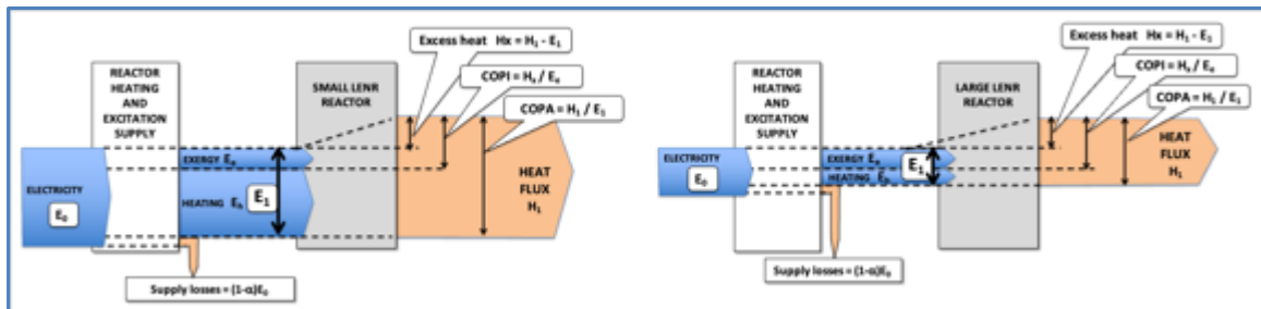
Comparison of the Intrinsic (COPI) and Apparent (COPA) Coefficients of Performance between small and large reactors characterized by different relative heat losses
