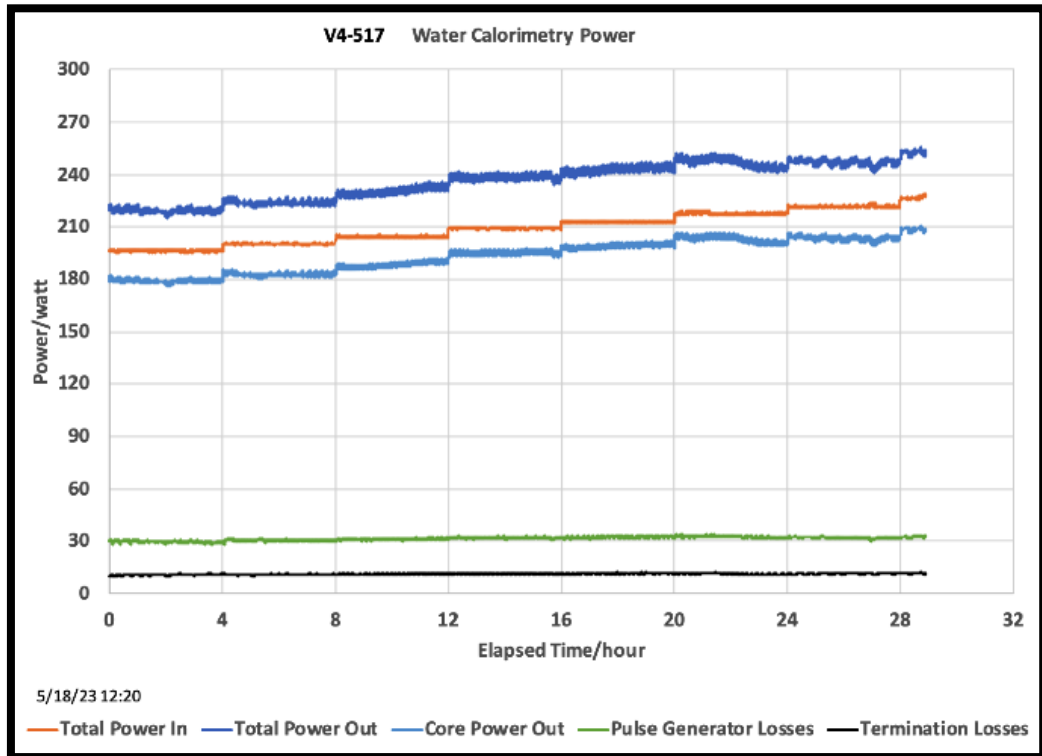
Figure 2. Input and output powers versus time during a Q-Pulse Run
