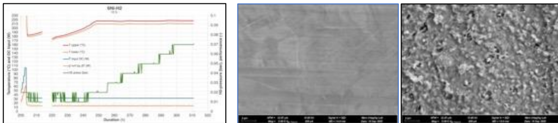
Fig. 1: Temperature effect Ni- Fig. 2a, b: SEM Ni foil before and after reaction
