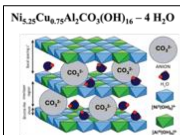
Structure of the hydrotalcite precursor
