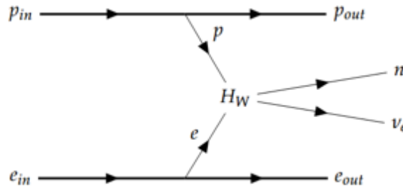
Figure 1. Feynman diagram for the coherent neutron production.
