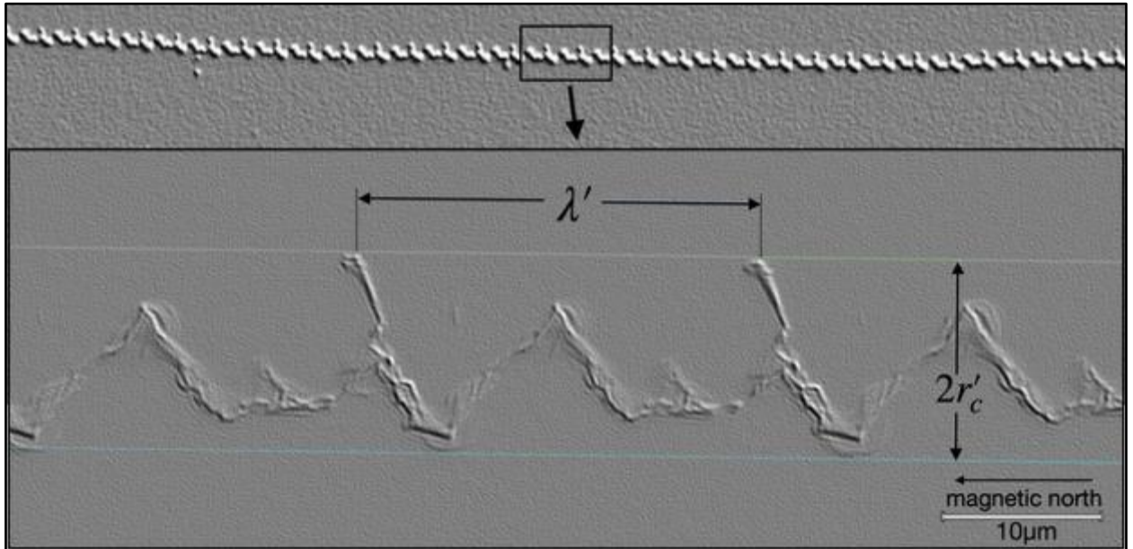
FIG. 1. Segment of 2663 \mu\text{m} track losing energy from right to left. Inset: Unit cell of \lambda'/r'_c = \phi = 25.59\mu\text{m}/6.52\mu\text{m} \approx 5\pi/4 .
