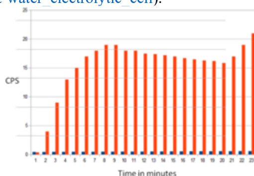
Figure 1. Trend of the counts for a test in the ARGAL laboratory in Bareggio for approximately 20 minutes from reaction activation.
