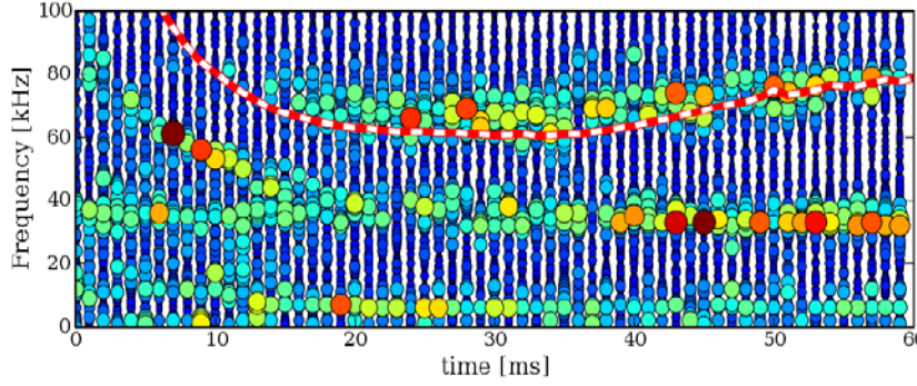
Fig. 10: Uppermost mode cluster (red dashed line) exhibits Helical Alfvén Eigenmode scaling as density varies in time for one plasma discharge.
