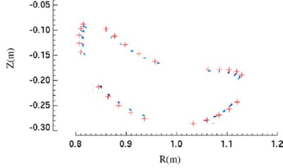
Figure 15: Measured vacuum punctures[+] and computation[+].
