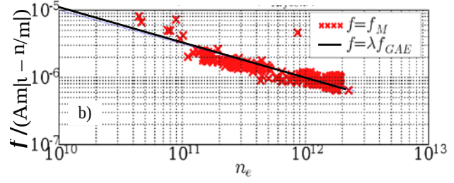
Figure 5: Reduced data showing clear Alfvénic dependence on 1/\sqrt{n_e} .
