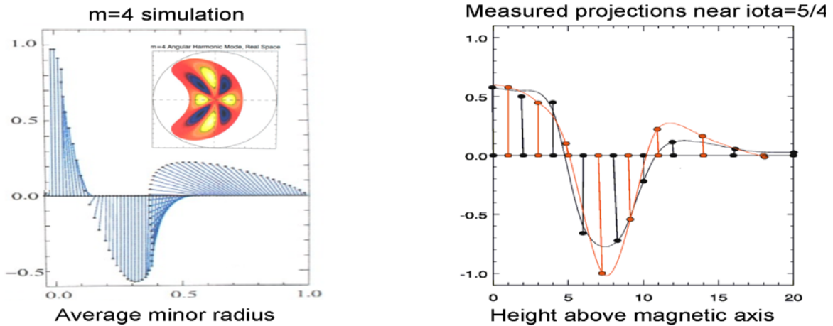
Fig. 12: a) Simulated and b) measured mode structure in line-integral density for the stronger modes near \iota=5/4 (large circles in Fig.11). The two scans shown are quite similar. The tilt of the phasors represents the phase angle. Chordal integration and symmetry causes phases to tend to 0 or \pi even for rotating modes.
