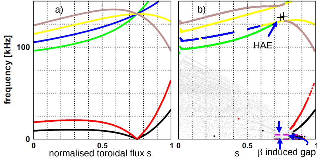
Fig. 9: CAS3D cylindrical (a) and 3D (b) frequency spectra. The grey dots are sound mode continua for high mode numbers, which need to be included for convergence, especially in H-1 which has a non-negligible mirror (bumpy) component in the 1/B^2 spectrum.
