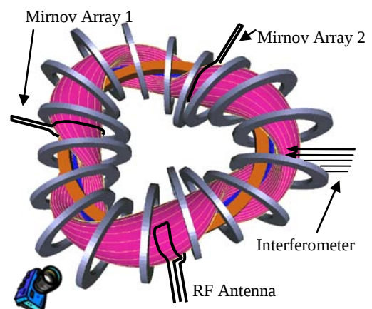
Figure 1: H-1 plasma showing location of Mirnov arrays, RF antenna, camera and interferometer; and 18 of 36 TF coils
