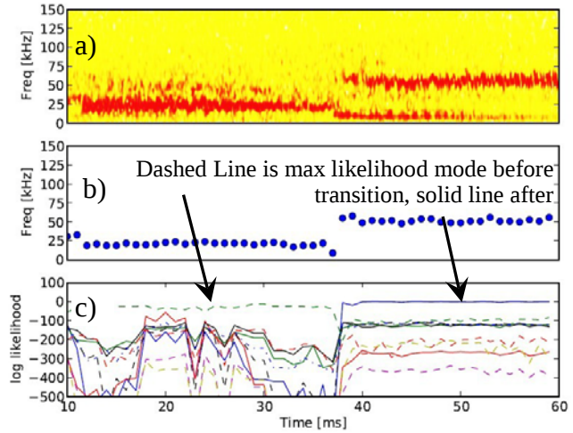
Figure 6: Spectrogram of MHD fluctuations in H-1, showing a) mode transition, b) mode extraction and c) identification.
