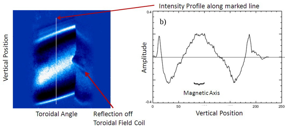
Figure 13: Phase-resolved side view of optical emission from MHD fluctuation in H-1 viewing between the toroidal field coils. A vertical section (b) along the line indicated shows an even mode
