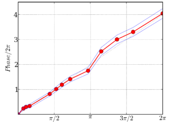
Fig. 8: Phase variation of the modes in cluster 6 with poloidal angle, showing a mode number m=4 . The red line and points show the cluster means, and the thin blue lines the standard deviation within the cluster.
