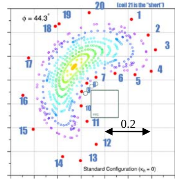
Figure 3 Coil position (1-20) and plasma at \phi = 44.3^\circ
