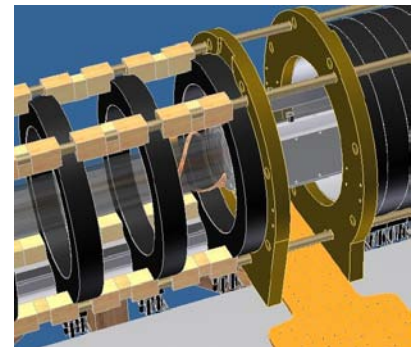
Figure 18: The materials diagnostic facility and b) close-up of the target chamber.
