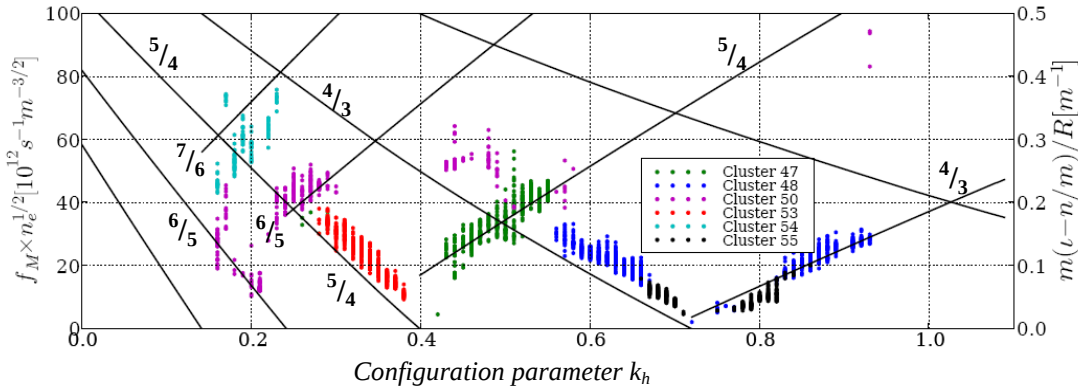
Figure 7: A more complete data set re-scaled by \sqrt{v_e} to show Alfvénic dependence on configuration parameter k_h . Lines show expected Alfvén frequency at the stationary point in rotational transform profile when the corresponding resonance is in the plasma, and at a fixed radius ( \langle a \rangle \sim 15\text{cm} ) if not.
