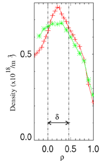
Figure 17: Plasma density increase in presence of an island (indicated by \delta ) for initial neutral densities of 0.8(+) and 1.6(*) 10^{18} \text{m}^{-3}
