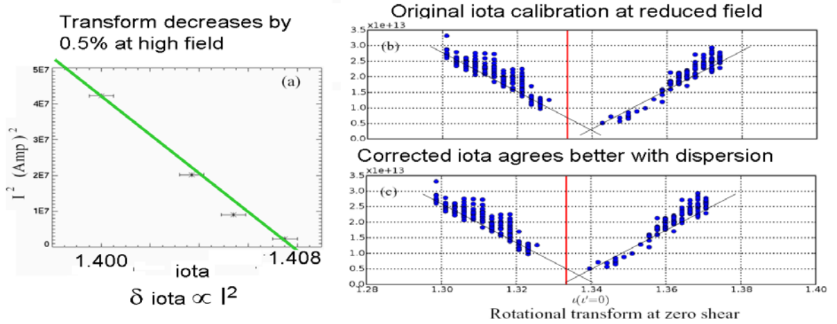
Figure 16 : Comparison of transform determination using Alfvén eigenmode resonance and direct ebeam mapping(a). The discrepancy between the transform obtained from the symmetry point in the “V” structure of the observed frequency (b) and the computed transform value is halved (c) if the computed transform is corrected for a small distortion in the magnetic field coils due to the magnetic forces inferred from the results (a) of electron beam mapping at high field.
