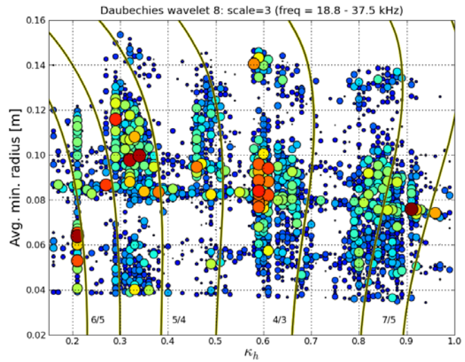
Figure 11: Dependence of line-averaged density fluctuation amplitudes (dot size) on effective radius of the line of sight and configuration parameter k_h . The swept nature of the diagnostic causes reproducible global modes (e.g. k_h \sim 0.6 ) to be artificially broken up into separate data points.
