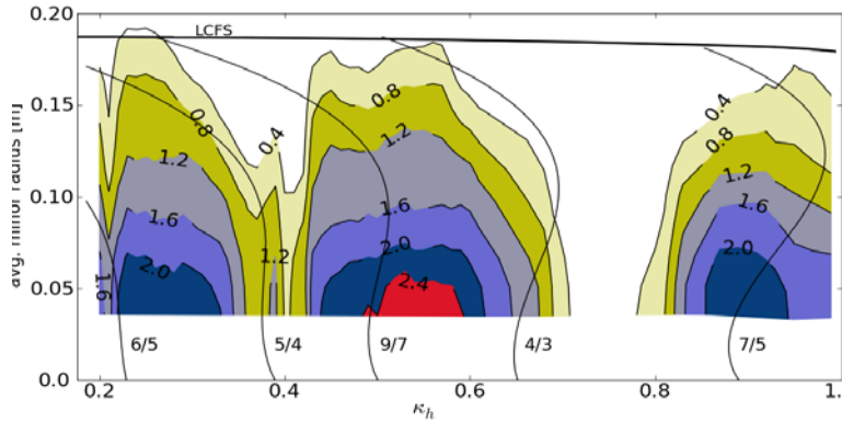
Figure 2: Contours of plasma density radial profile as configuration is varied.
