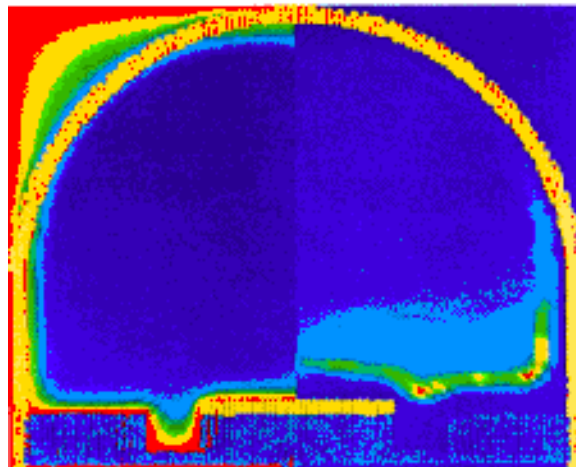
Fig. 3.3-1. Discharge in a realistic geometry using the FLIP code [74]. On the left, the electrostatic potential is shown (yellow: 50V, purple: -10V). On the right the dust density is shown, illustrating how the geometry of the base can be used to design cleaner plasma reactors.
