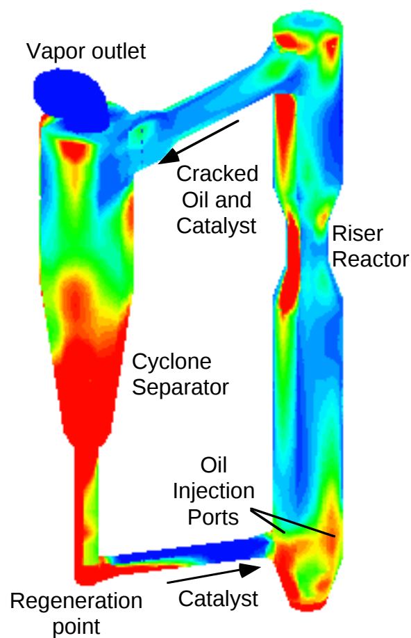
Fig. 3.2-1. One time in a simulation of the startup and operation of a recirculating fast-fluidized bed (FFB) reactor using CFDLIB with multiple fields and phases. The colors reflect the local volume fraction of the solid catalyst (red-high, blue-low).
