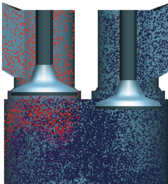
Fig. 3.1-1. A color visualization of the temperature field during the inlet flow in a hydrogen-fueled engine simulated with KIVA-3 [62][90]. The open intake valve is on the right; the closed exhaust port is on the left. The particles are used only to simulate the flow and are colored according to the temperature of the gas. The cold intake air (blue) is shown compressing the residual hot combustion gases (red).
