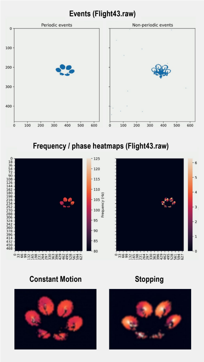
Figure 16: (top) Separation of periodic from non-periodic EBS drone data. (middle) Quantitative assessment of rotor frequency (left) and phase (right), providing characterization information for the periodic clusters. (bottom) Frequency changes corresponding to changes in drone motion.
