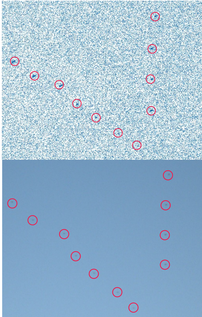
Figure 12: Data collected from an EBS (top) and a conventional framing camera (bottom). Both images show the same scene at roughly the same time. The system accumulated event data into a frame for visualization (blue corresponds to an event; white corresponds to “no data”). Red circles, added manually, mark the locations of the drones.
