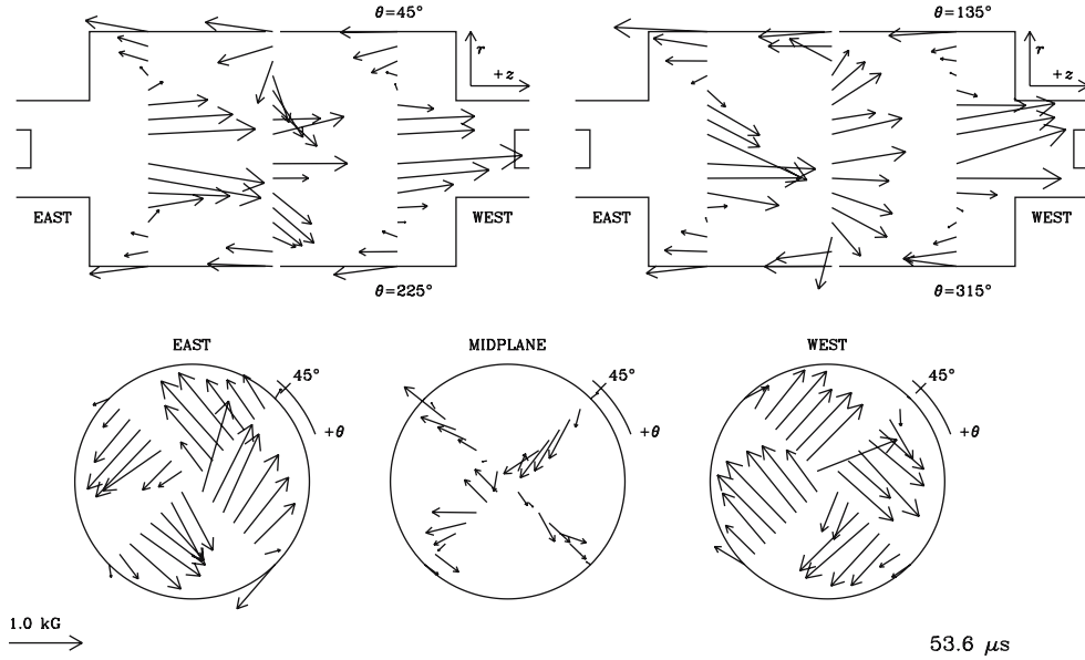
Fig. 2. Global magnetic structure. Five views of the data are shown: two orthogonal rz projections (top row) and three r\theta projections (bottom row) at t = 53.6 \mu\text{s} . The scale of 1 kG is indicated bottom left.
