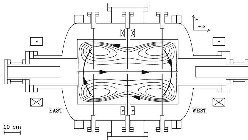
Fig. 1. The Swarthmore Spheromak Experiment (SSX) as configured for counter-helicity spheromak merging experiments, and flux surfaces for a Grad-Shafranov equilibrium for incomplete poloidal flux reconnection.
