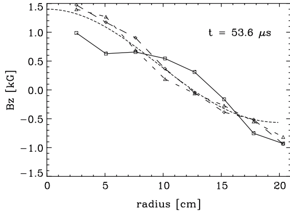
Fig. 3. Toroidally averaged B_z radial profile for the east, mid-plane, and west probe positions (diamond, square, and triangle plotting symbols, respectively). The force-free spheromak Bessel model (dotted) compares favorably to the east and west data. The field null at r_0 \approx 14 cm for the midplane data is consistent with the simple FRC prediction r_0 = R_s/\sqrt{2} .
