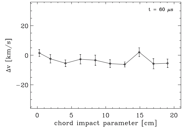
Fig. 5. Chord-averaged ion flow as a function of chord impact parameter after spheromak merging is complete. For comparison, the Alfvén velocity is \approx 100 km/s.
