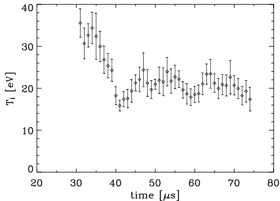
Fig. 4. Ion temperature averaged over 10 merging experiments. The IDS view chord for this measurement is along a diameter at the midplane. Large temperatures prior to t = 40 \mu s are likely due to the gun discharge, while the marginal \approx 10 eV increase after t = 40 \mu s may be due to reconnection.
