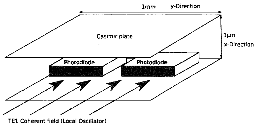
Figure 16. Diagram of Casimir Cavity with BHD Photodiodes. (courtesy of P. Marecki)
