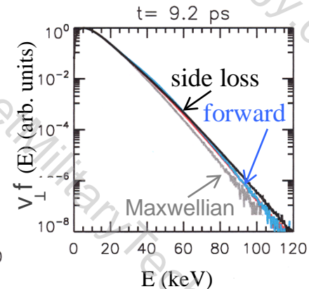
Hot e flux without B_x field
