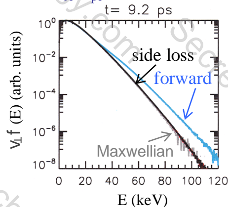
Hot e flux with B_x field \Omega_{ce}/\omega_{pe} = 0.01 t = 9.2 ps
