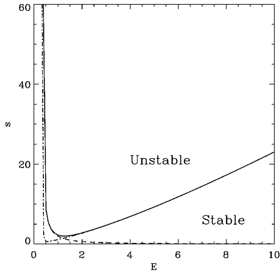
FIG. 8. Stability diagram in s and elongation with stabilizing effects from ion gyro-viscosity.
