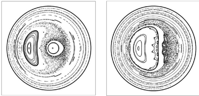
Figure 6: An example of Reverse field pinch fields computed generated by the SPEC code. The left image shows a double axis and the right a single helical axis.
