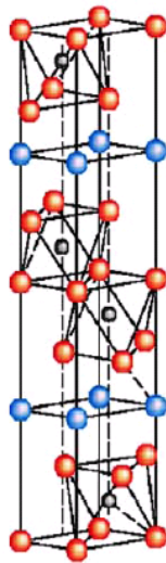
Figure 7: The structure of \text{Ti}_3\text{SiC}_2
