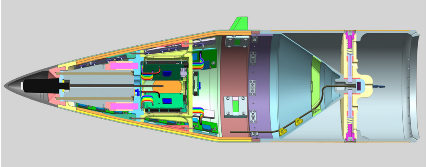
Side view drawing of STAJe- Phase 1 flight vehicle, designed to develop a pipeline of trained people in high speed flight testing as well as to explore different approaches to increase the frequency of flight testing at reduced cost. This program is being undertaken at the University of Queensland with the assistance of AIMTEK, Hypersonix, Lockheed Martin Australia and in collaboration with BlackSky Aerospace. It was due to fly in May 2024. Phase 2 and 3 of STAJe- will demonstrate high speed (Mach 2–4) electric propulsion by 2026
