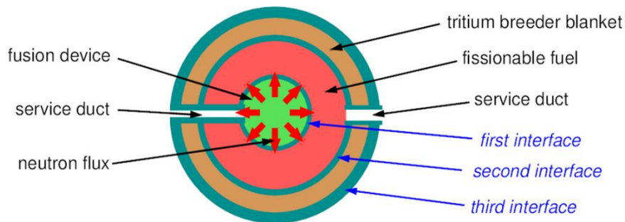
Figure 1: Scheme of a FFHR reactor
