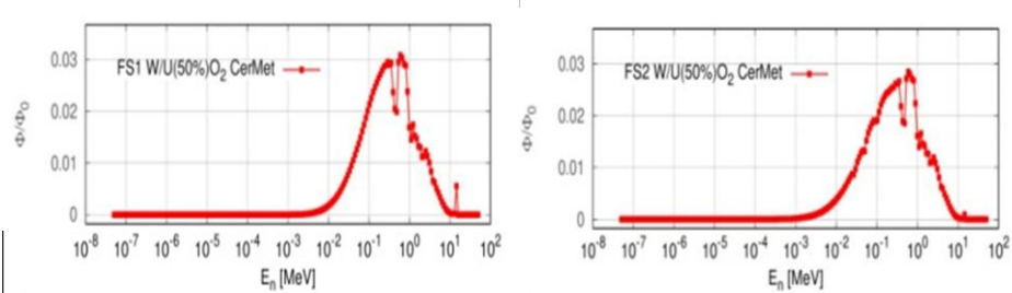
Figure 2: Neutron spectra for shell 1 and shell 2, using CerMet W/[U (50%) O 2 ] in both.
