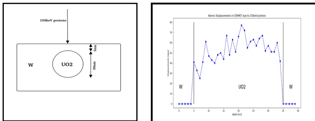
Figure 3: scheme (left) and damage in the Cermet (right), using IMPC5 simulation
