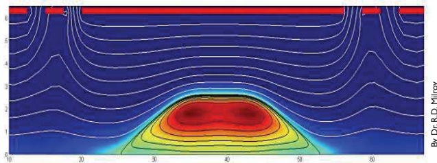
Moqui (2D) simulation of the translated FRX-
