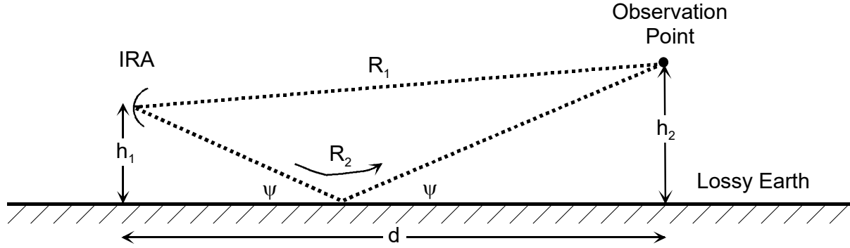
Figure 20. Illustration of the IRA located over a lossy earth.
