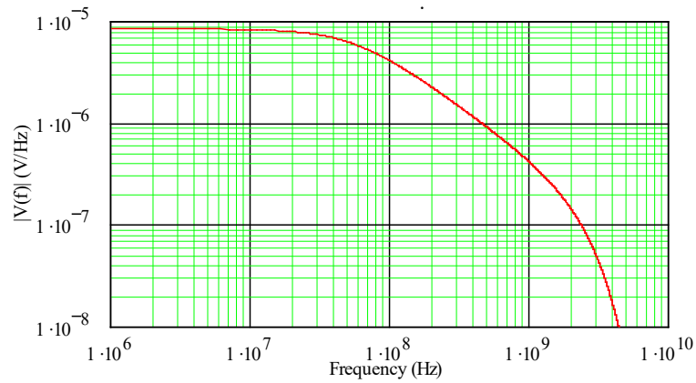
Figure 17. Plot of the frequency domain spectrum magnitude for the pulser output voltage of Figure 8.
