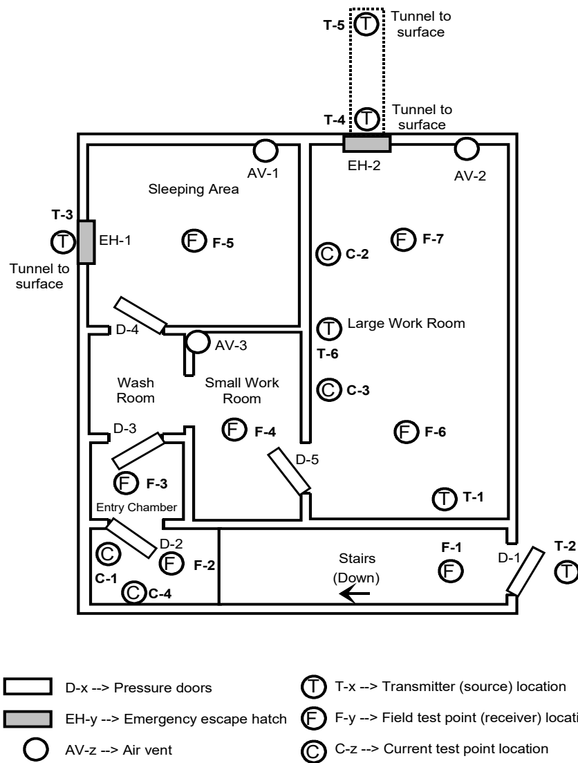
Figure 12. Transmitter and measurement locations for the buried test facility.
