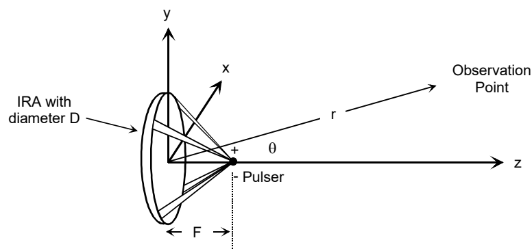
b. Illustration of the antenna
