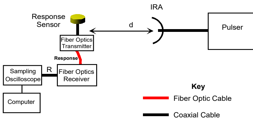
Figure 4. Equipment configuration for transient IRA characterization (MG-2).
