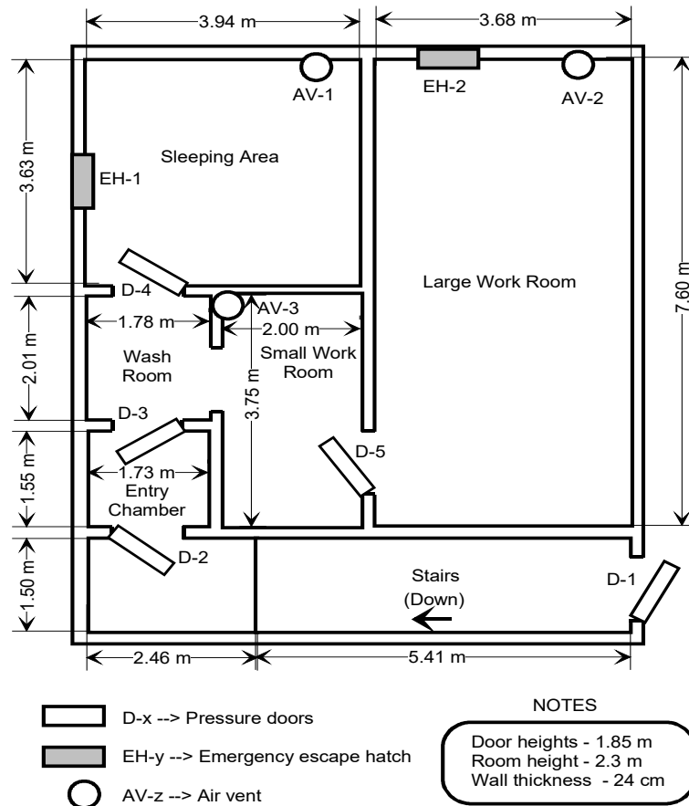
Figure 2. Floor plan and dimensions of the testbed buried facility at the Swiss NEMP Laboratory in Spiez.
