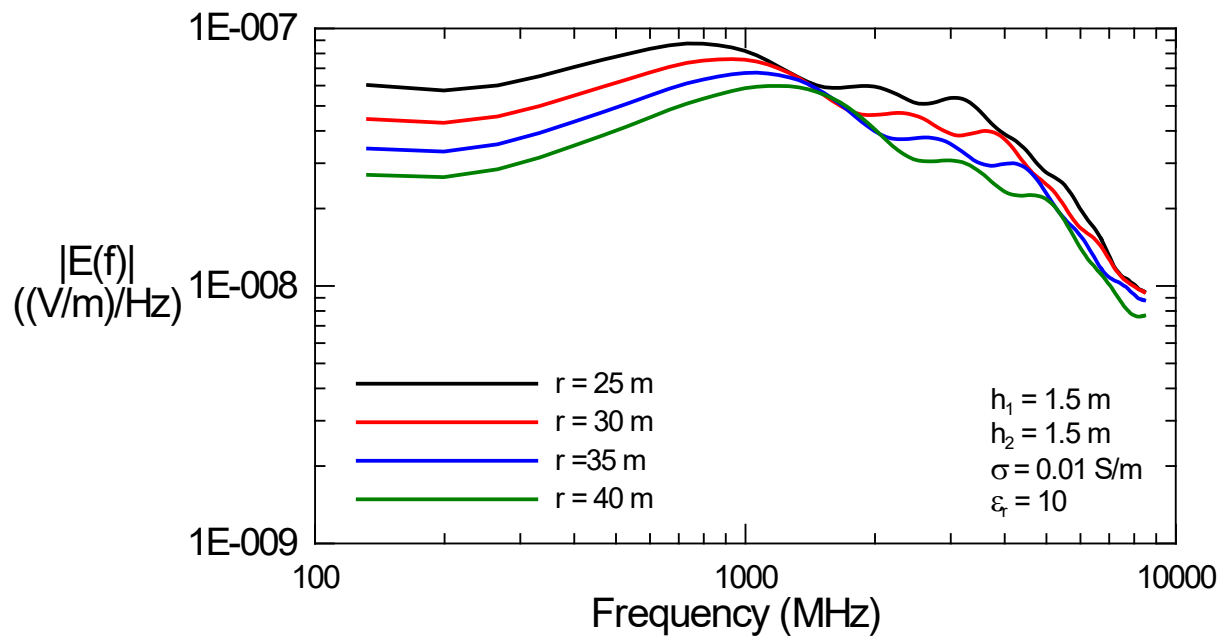
d. Spectral response for d = 25 to 40 \text{ m}
