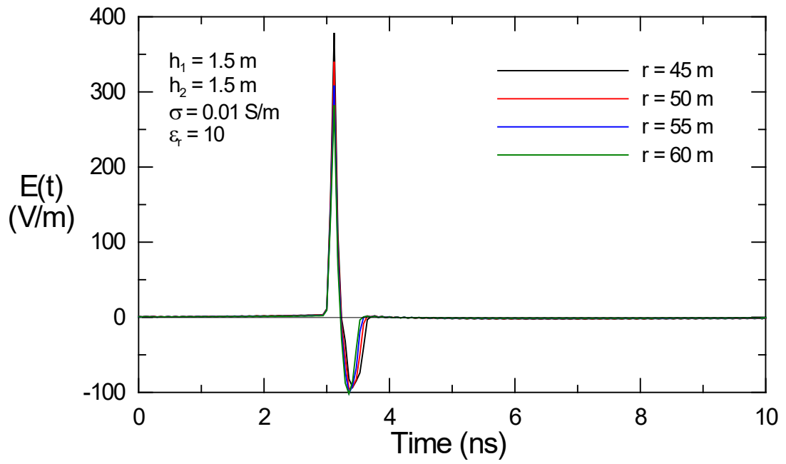
e. Transient response for d = 45 to 60 m
