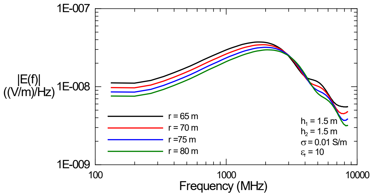
h. Spectral response for d = 65 to 80 m
