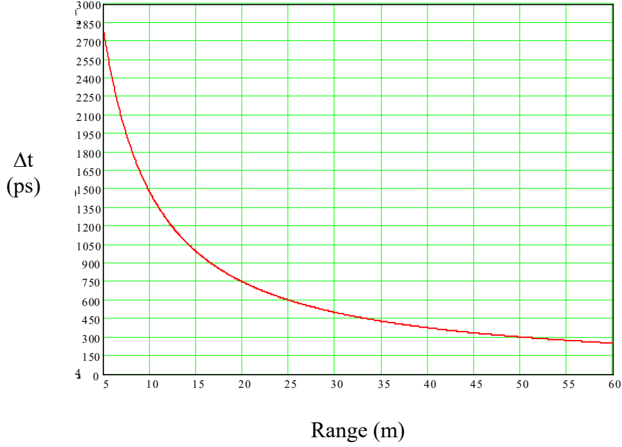
Figure 21. Plot of the time difference in arrival of the earth-reflected pulse relative to the direct pulse. (From ref.[1]).
