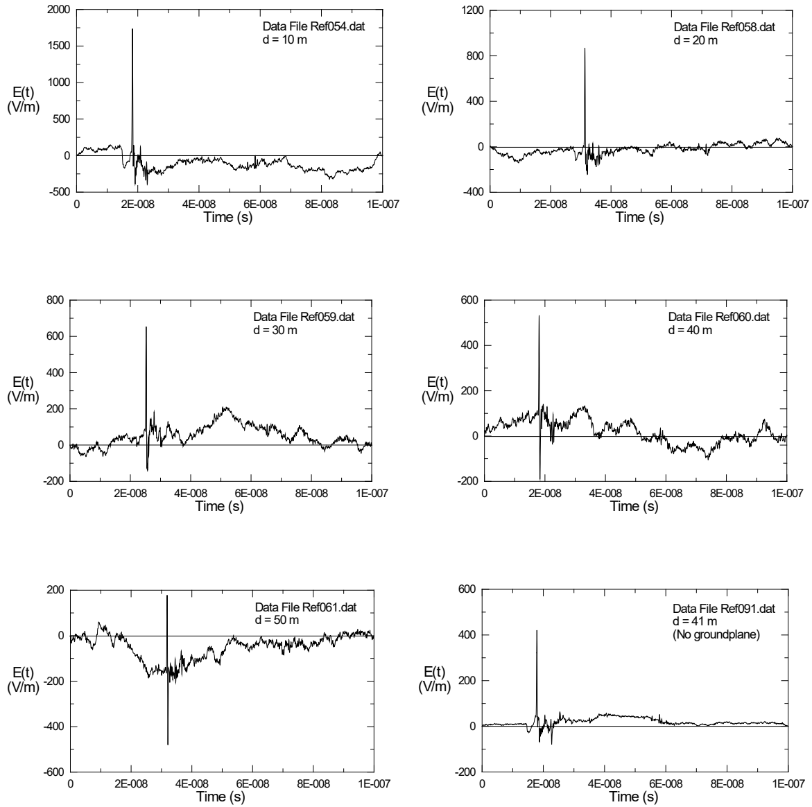
Figure 19. Plots of measured IRA E-fields at different ranges from the antenna.
