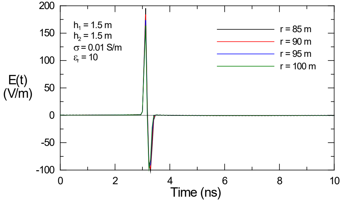
i. Transient response for d = 85 to 100 m
