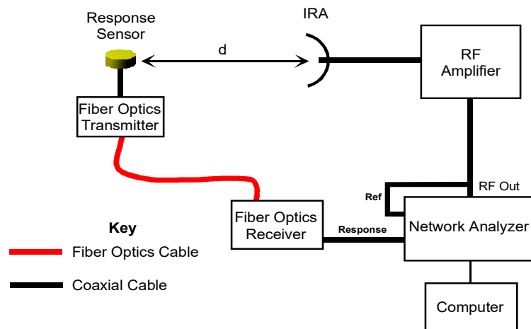
Figure 5. Equipment configuration for CW IRA characterization (MG-3).
