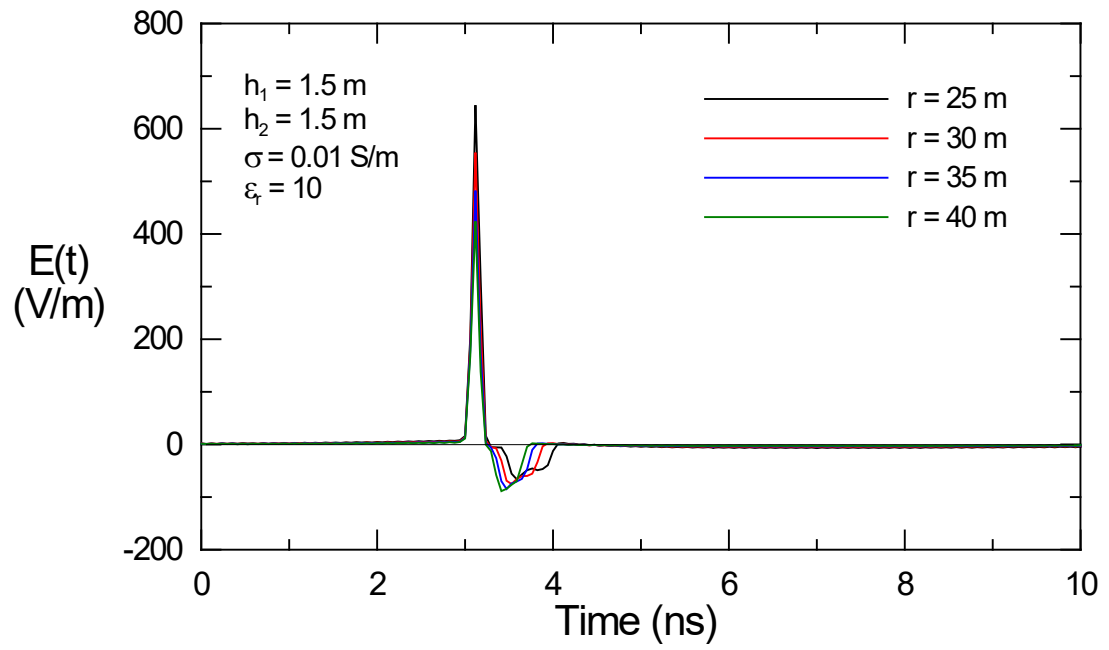
c. Transient response for d = 25 to 40 \text{ m}
