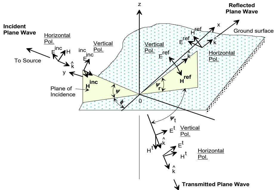
Figure 1. Reflected and transmitted waves at the air-earth interface
