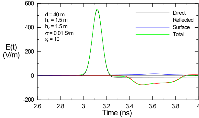
Figure 23. Illustration of the various wave contributions to the total E-field from the IRA at a distance of 40 m from the IRA for an earth conductivity of \sigma = 0.01 S/m and a relative permittivity \epsilon_r = 10 .
