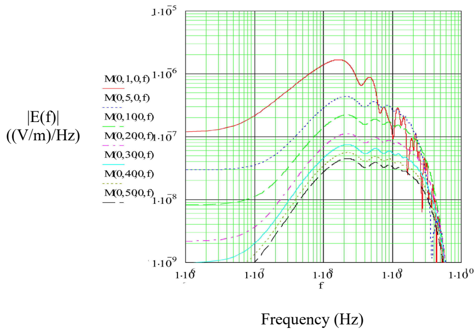
Figure 10. The computed spectral magnitude of the IRA on-axis E-fields of Figure 9.
