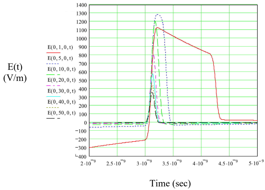
Figure 9. Plot of the computed on-axis IRA transient E-field (in V/m), shown for various ranges from the antenna.
