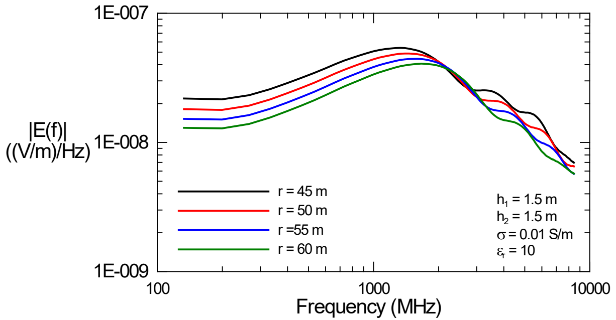
f. Spectral response for d = 45 to 60 m
