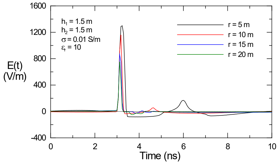
a. Transient response for d = 5 to 20 \text{ m}
