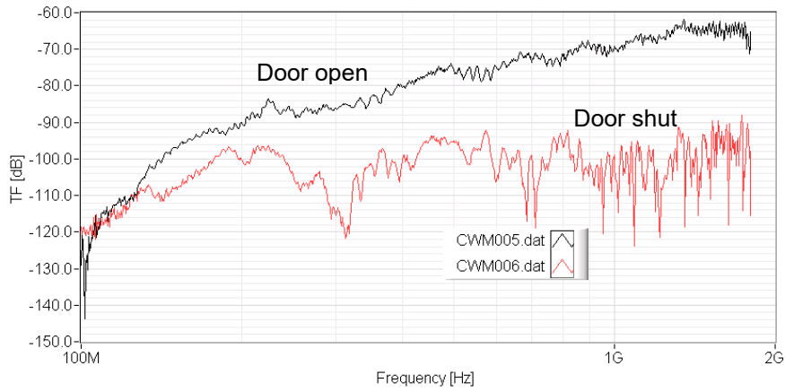
a. Unprocessed measured transfer function data.
