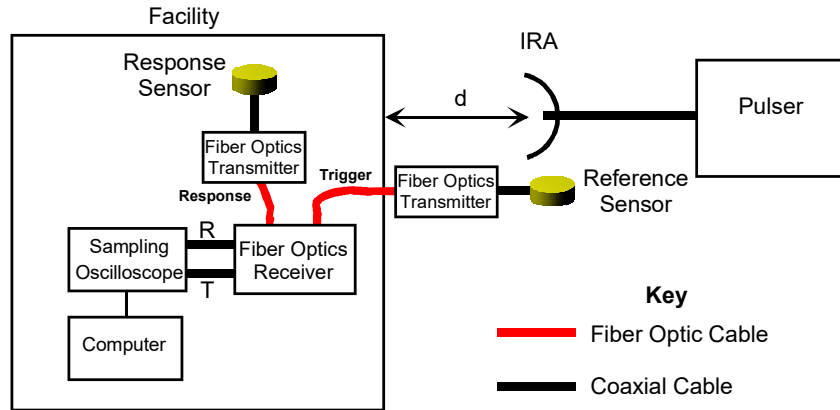
(a) Transient measurements
