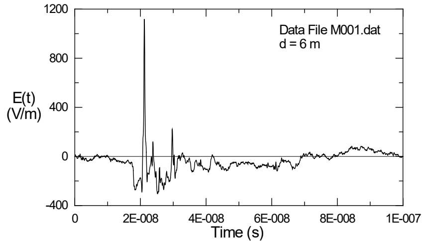
Figure 11. Measured transient equivalent E-field from the IRA at 6 m from the antenna.
