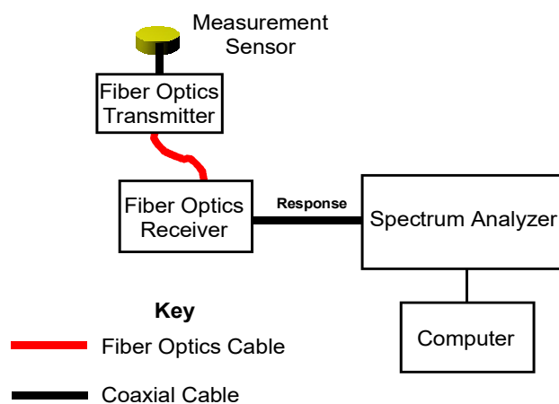
Figure 3. Equipment configuration for ambient noise measurements (MG-1).
