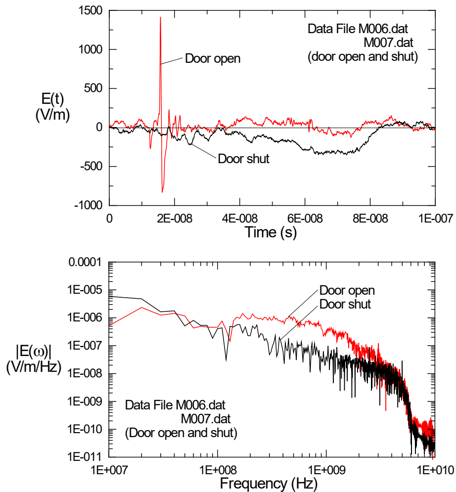
Figure 14. Measured (equivalent) transient E-field inside the main facility door (top) and the corresponding spectral magnitude (bottom) for the IRA in the position shown in Figure 13, with the door open (data record M006.dat) and the door shut (record M0007.dat).
