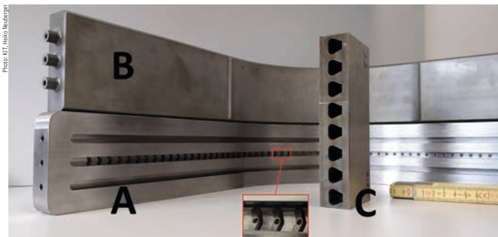
A) Semi-finished product: preformed shell with surface-milled channels including internal structuring (so-called semi-detached ribs) in the center channel. B) Component after sealing the channels with HMG's MPA process. C) Section through a demonstration part
