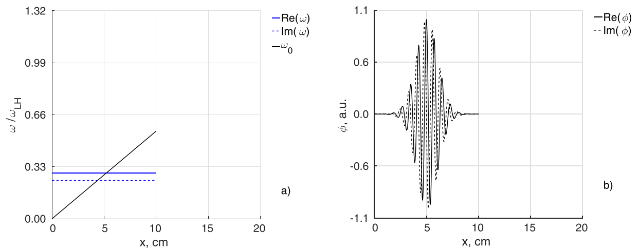
FIG. 11. The eigenfunction with largest growth rate \omega = (0.29 + 0.24i) \cdot \omega_{LH} \text{ s}^{-1} , k_y = 100 \text{ m}^{-1} , L = 10 \text{ cm} .
