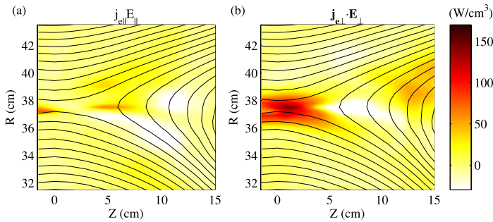
Fig. 10 Comparison of two compositions of energy deposition rate measured in MRX for symmetric, anti-parallel magnetic reconnection; (a) j_{e\parallel} E_{\parallel} and (b) j_{e\perp} \cdot E_{\perp} . Figure from Yamada et al. (2016)
