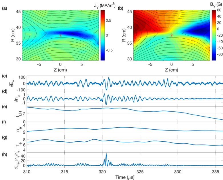
Fig. 15 Measured ES-LHDWs. (a,b) Out-of-plane current or magnetic field component (color) with the poloidal flux contours (black lines) representing the magnetic field lines at 326 \mu s. The red asterisk indicates the location of the probe. The upper side ( R > 37.5 cm) has a higher density. (c) Time series of \delta E_{rec} in V/m. Wave activity near the lower hybrid frequency ( f_{LH} \sim 2 MHz) is detected while the probe stays near the reconnection site. The amplitude of the fluctuation is comparable to the mean reconnection electric field ( \langle E_{rec} \rangle \sim 100 V/m). (d) Time series of \delta n_e in 10^{13} cm -3 during the quasi-steady reconnection period. Time series of f_{LH} (e), averaged density ( \langle n_e \rangle ) in 10^{13} cm -3 (f), and electron temperature ( T_e ) in eV (g) are shown. A sharp decrease of f_{LH} is observed with the approach of the X-point to the probe. Time series of \delta E_{rec} \delta n_e / \langle n_e \rangle are shown in (h). Positive correlation between \delta E_{rec} and \delta n_e indicates that the wave is capable of generating anomalous resistivity. Figure from Hu et al. (2021)
