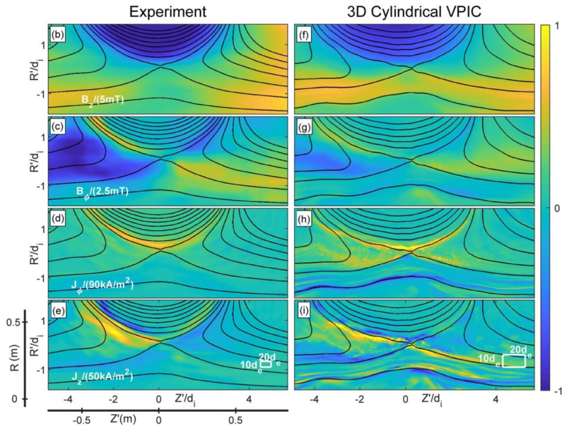
Fig. 7 (Panel b-e) Magnetic field and current components recorded in TREX during reconnection. (Panel f-i) Matched 3D kinetic simulation results reproducing the experimental results. After Greess et al. (2021)
