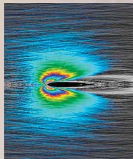
Wake potential of a fast charged-ion projectile in a dense plasma background.
