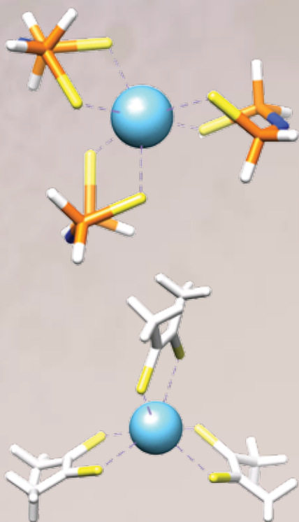
Coordination geometries of lanthanum to imidodiphosphinochalcogenide (top) and dithiolene (bottom).
