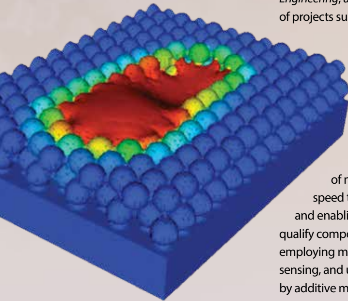
Simulation of laser melting of a powder layer showing consolidation by surface tension and gravity and the molten pool in the middle.
