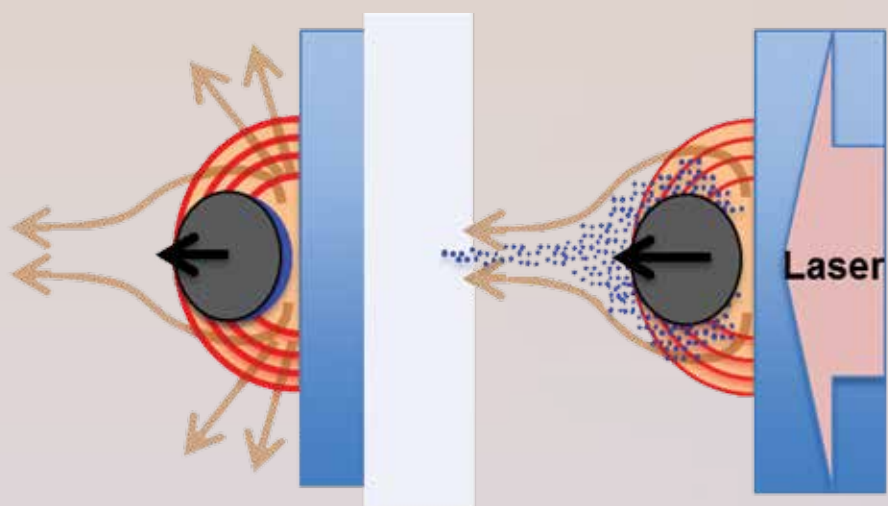
Laser ablation of idealized spherical metal contaminants from fused silica optics, shown schematically and captured using nanosecond pump–probe imaging. Significant material spall is observed, which can degrade the optic.
