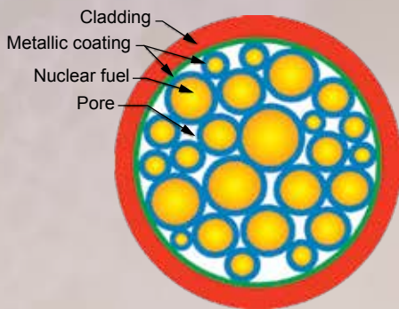
Schematic of an inert metal matrix fuel.
