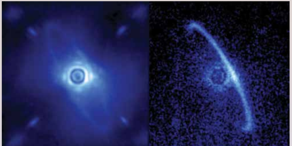
Gemini Planet Imager's first-light image of a dust disk around the star HR4796A, in total infrared intensity (left) and polarized light (right). Image courtesy of Gemini Observatory, and image processing by Marshall Perrin, Space Telescope Science Institute.
