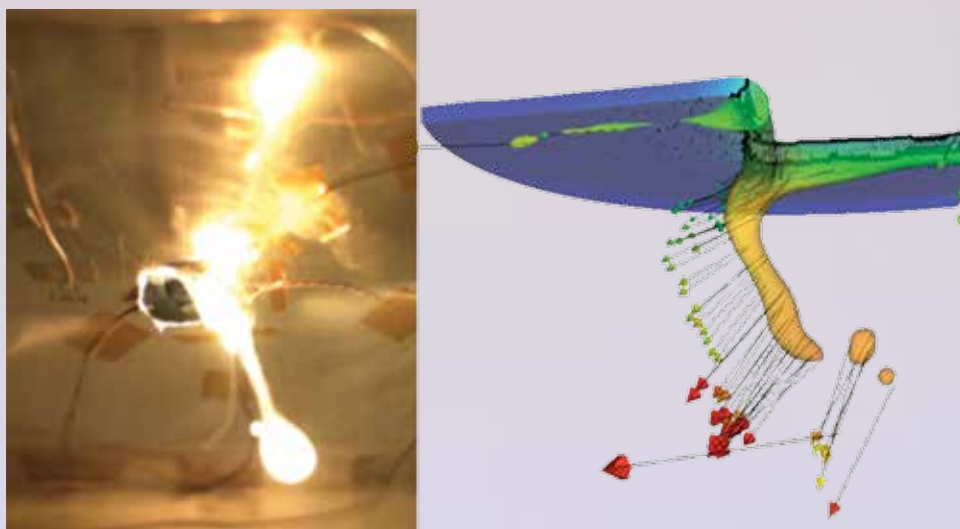
A melt blob formation for a 1-mm aluminum sheet irradiated at 200 \text{ W/cm}^2 , in which the blob itself can damage sensitive elements in a target. On the right, the modeling results for similar conditions. Arrows indicates the melt velocity.
