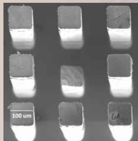
Tall silicon mirrors (aspect ratio of 1:7) for back-reflecting high-intensity x-ray pulses. The center mirror had been exposed to an x-ray free-electron laser pulse and was obliterated, while the surrounding pillars were not affected.
