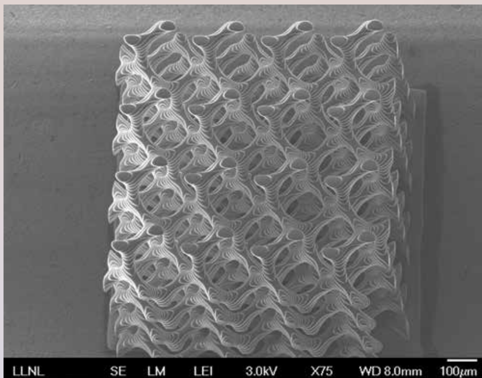
Scanning electron microscopy image of a three-dimensional printed micro-battery architecture. The architecture material is a lithium-ion solid-state electrolyte. The architecture design consists of two discrete but interpenetrating channels designed to reduce transport distances between the active material phases (i.e., anode and cathode).
