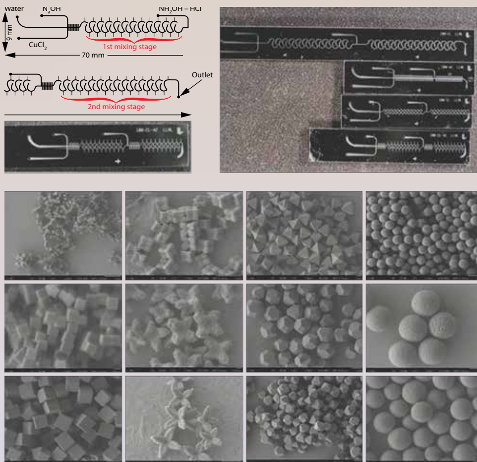
Schematic and images of our micro-mixers used for advanced material synthesis (top) and scanning electron microscopy images of copper oxide nanometer-scale particles with a diverse morphology used to test the feasibility of these particles as feed materials for additive manufacturing (bottom).
