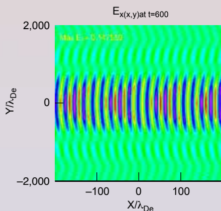
A traveling electron plasma wave undergoing simultaneous self-focusing and longitudinal modulational instability.
