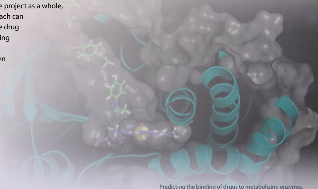
Predicting the binding of drugs to metabolizing enzymes.
