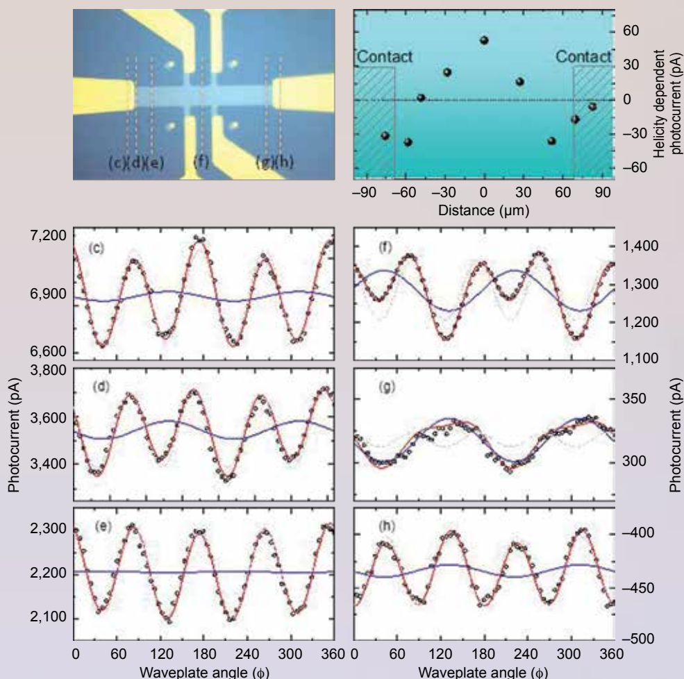
Photocurrents induced on the surface of a 10-nm topological insulator film using an infrared laser. An optical image of topological insulator devices is shown top left. Photon polarization-dependent photocurrent as a function of laser spot position is seen top right. The measured photocurrent versus quarter-waveplate angle is shown in the six charts. The blue curve depicts polarization-dependent photocurrent.
