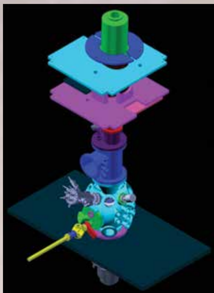
The new LION (laser ionization of neutrals) instrument, currently under construction at LLNL to accelerate the pace of development for applying resonance ionization mass spectrometry to characterization of nuclear materials. The LION is a 2-m time-of-flight mass spectrometer, specifically designed to measure ions created by laser ionization of secondary neutral atoms.
