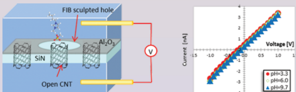
Schematic representation of the experimental setup used to study electric-field-driven molecule translocation through a single carbon-nanotube channel (left). Example of a linear current–voltage response of a carbon-nanotube fluidic channel filled with ionic solutions at three different pHs (right).
