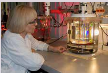
Lawrence Livermore physicist and LDRD researcher Natalia Zaitseva examines a single crystal growing in a solution-growth crystallizer developed for production of stilbene crystals for fast neutron detection.
