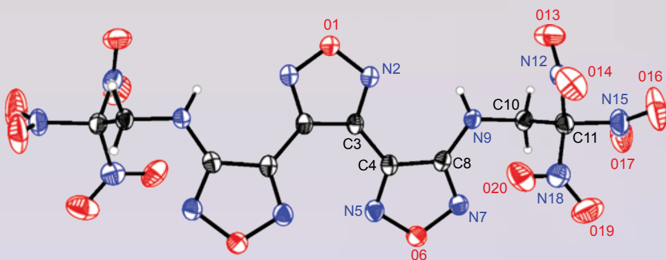
Crystal structure of our newly developed energetic compound LLM-204.
