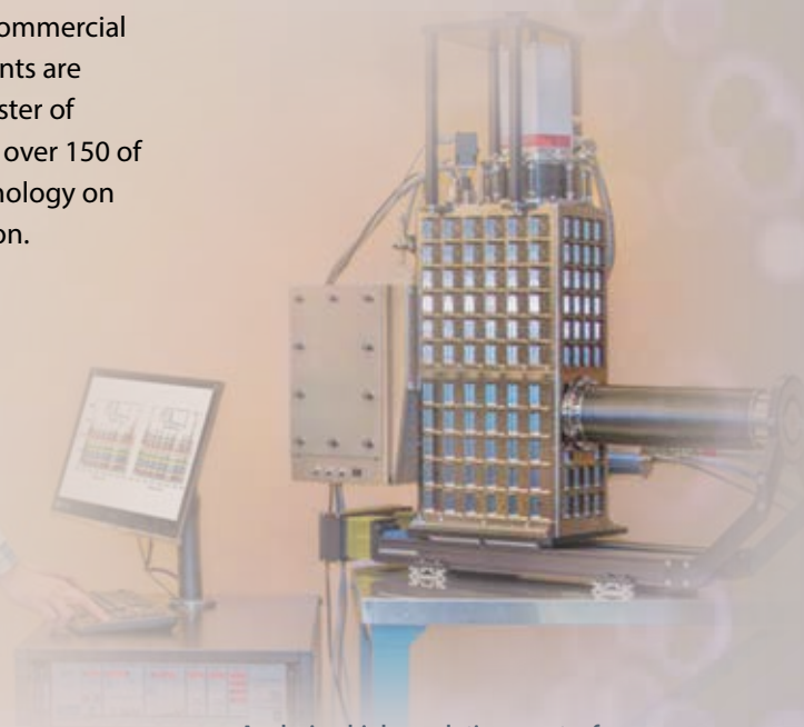
Analyzing high-resolution spectra from the superconducting tunnel junction x-ray spectrometer (shown on the table) to characterize a material sample. The rack contains support electronics for spectrometer operation. (Photo by Roy Kaltschmidt of Lawrence Berkeley National Laboratory.)
