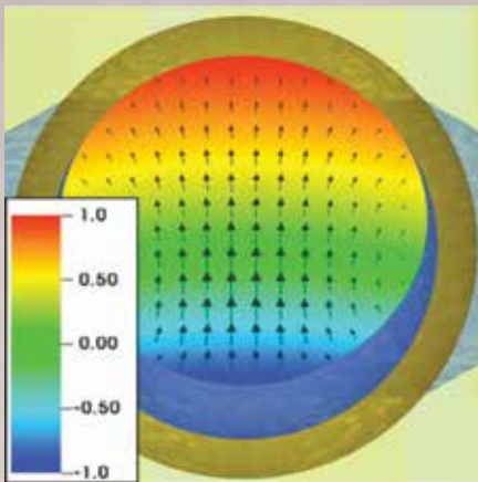
Computed evaporation-driven velocity field in the hydrogen vapor (shown as arrows) for research into the growth of high-quality hydrogen layers used for laser fusion research.
