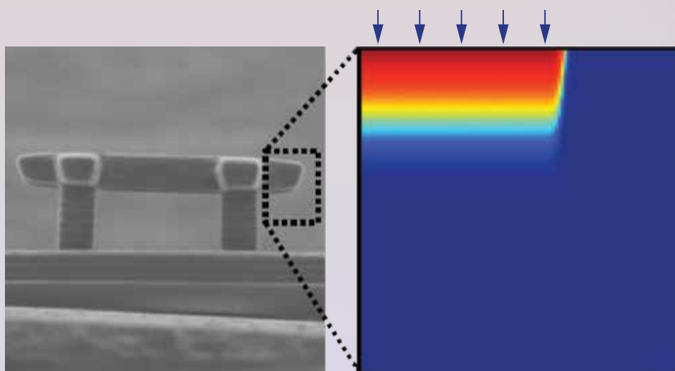
Comparison between a bridge structure overhang fabricated with stereolithography to the computed profile from the process model. Colors in the model indicate the amount of polymerization (blue, which is uncured, to red, which is fully polymerized).
