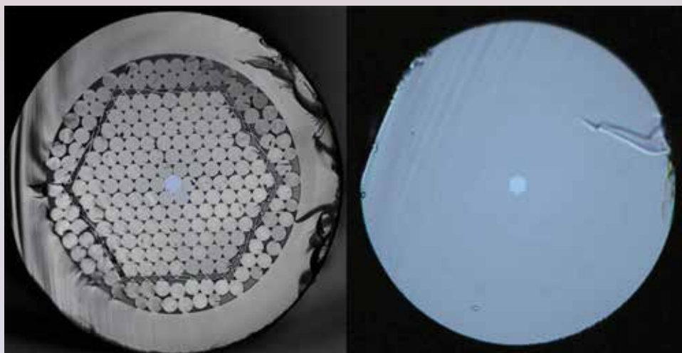
The laser fiber on the left shows an intermediate stage in the process of drawing the preform starting materials to the finished fiber. At the center is the neodymium-doped core, which is the lasing medium. The outer hexagon allows an air gap into the fiber cross section, forming a confining pump-light cladding. The image on the right shows the finished fiber, in this case without cladding.
