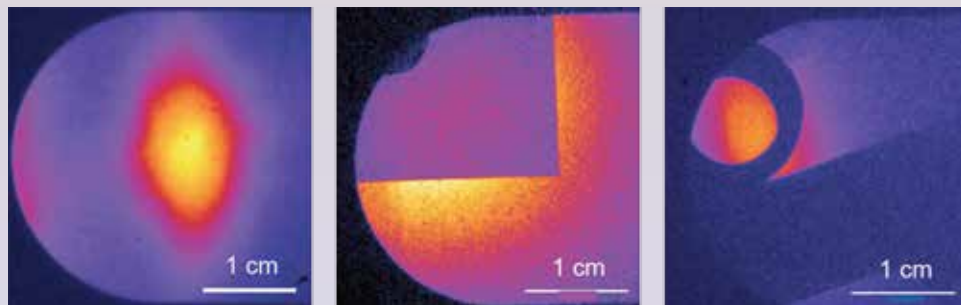
Betatron x-ray radiographs obtained at the Jupiter Laser Facility in Livermore reveal images of a laser beam profile (left), silicon wafer (center), and gold ignition target capsule (right).
