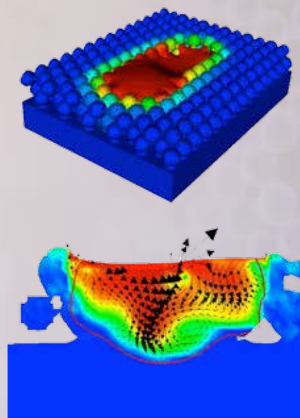
Simulation laser melting of a powder layer containing a hexagonal array of 27- \mu\text{m} -diameter stainless-steel powder particles shortly after the laser was turned off, showing consolidation by surface tension and gravity. The color represents temperature. The molten pool is visible at top and the recirculation of the liquid metal is represented by the arrows in the cross section at the bottom.
