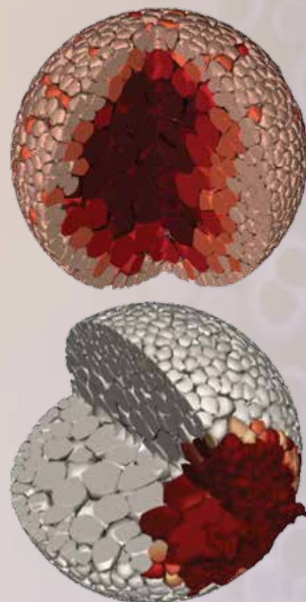
Initial configuration of a hypothetical asteroid with a section removed to view the interior structure (top). Colors designate different size ranges of boulders. Snapshot of early-time response to energy deposition from a nuclear blast on the front surface, with colors representing velocity magnitude (bottom).
