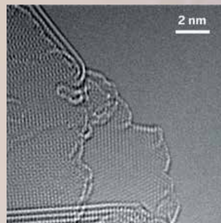
A high-resolution transmission electron micrograph reveals highly ordered carbon atoms within the layers of a graphene aerogel.
