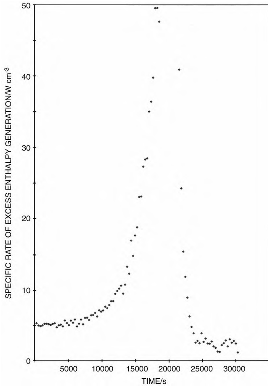
Fig. 22. Comparison of specific rates of excess enthalpy generation, \text{Wcm}^{-3} , on day 68 during the period 0 < t < 21,300 \text{ s} and the initial period 21,300 \text{ s} < t < 30,300 \text{ s} of observation of "Heat after Death."
