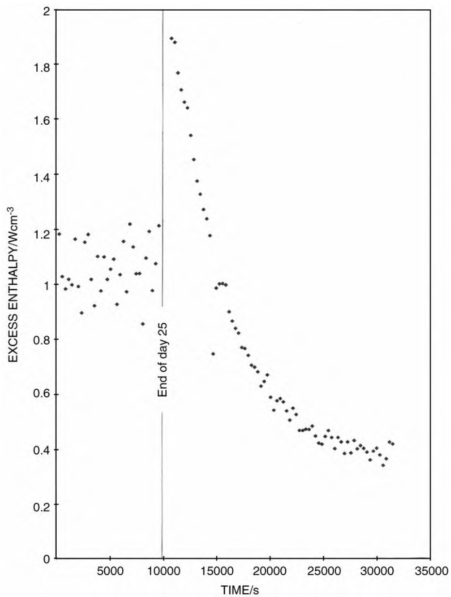
Fig. 25 The specific rate of excess enthalpy generation, \text{Wcm}^{-3} , for the last part of operation on day 25 and the first part on day 26.
