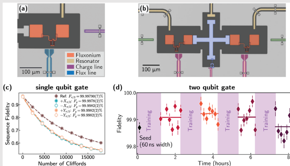
Figure 3.7: (a) Device image for leading 1 qubit error on fluxonium. 143 (b) Device image for a high fidelity two-qubit gate with fluxonium. 144 (c) Example data from (b), illustrating the achieved 1-qubit gate fidelity exceeding 99.9978% and (d) 2-qubit gate fidelity exceeding 99.9% (Error % = 100 % - fidelity %).
