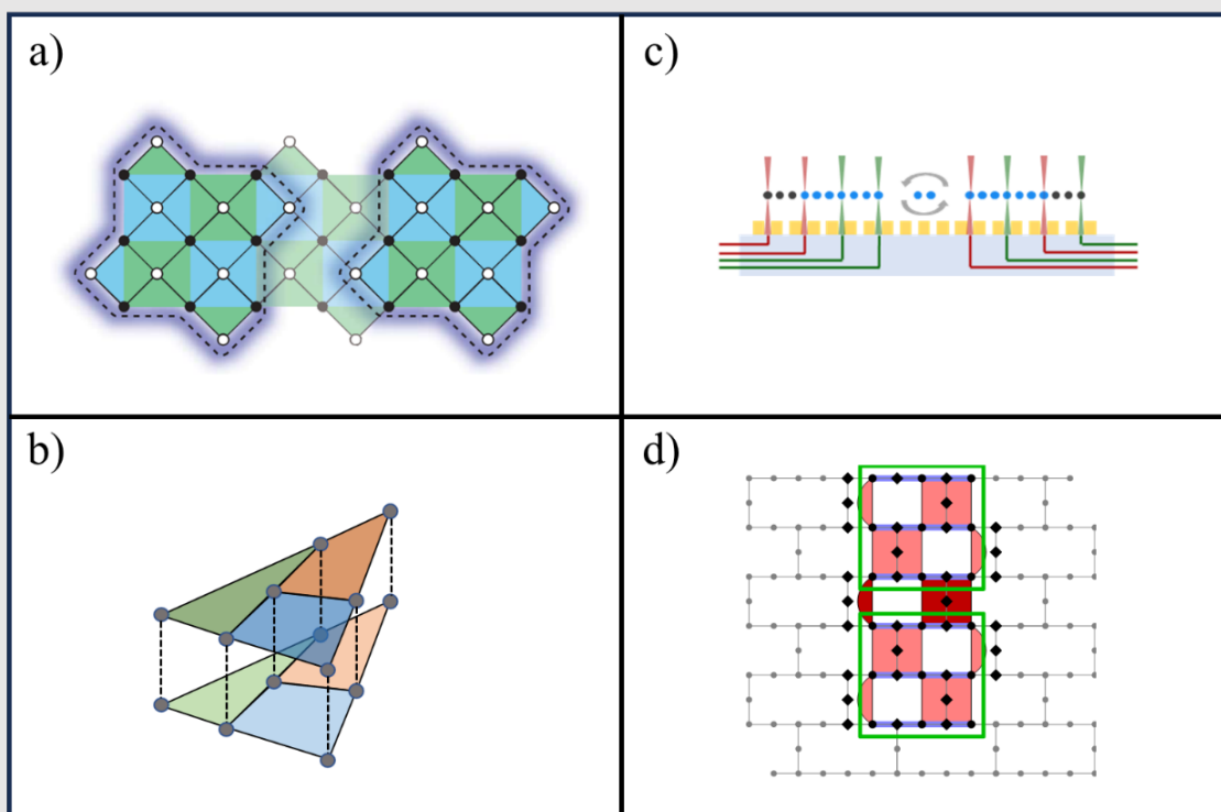
Figure 3.8: ELQ's logical-qubit entanglement concepts. (a) Logical entanglement concept based on the surface code and the lattice surgery approach, to be realized separately using fluxonium and transmon qubits. (b) Applying transversal gates between copies of the Steane (color) code, made with neutral-atom qubits. (c) Logical qubit entanglement using the lattice surgery approach between color codes in trapped-ion systems incorporating integrated optics. (d) Lattice surgery concept based on the so-called heavy-hex code, to be implemented on a transmon-based quantum computer. 146
