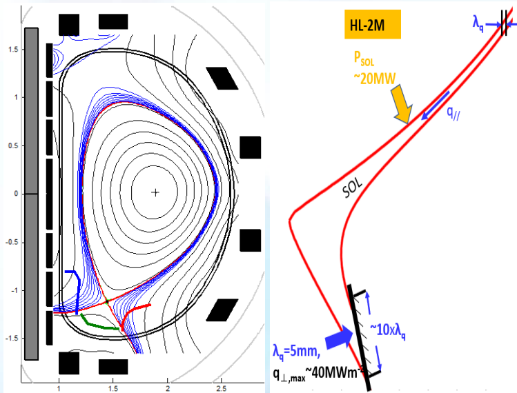
Standard divertor
