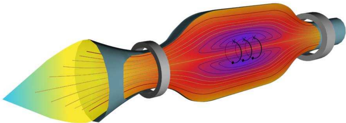
Fig. 2. Mirror nozzle, mirror coils and direct energy conversion (DEC) system for the prolate FRC (racetrack) as magnetic fusion rocket (space propulsion)
