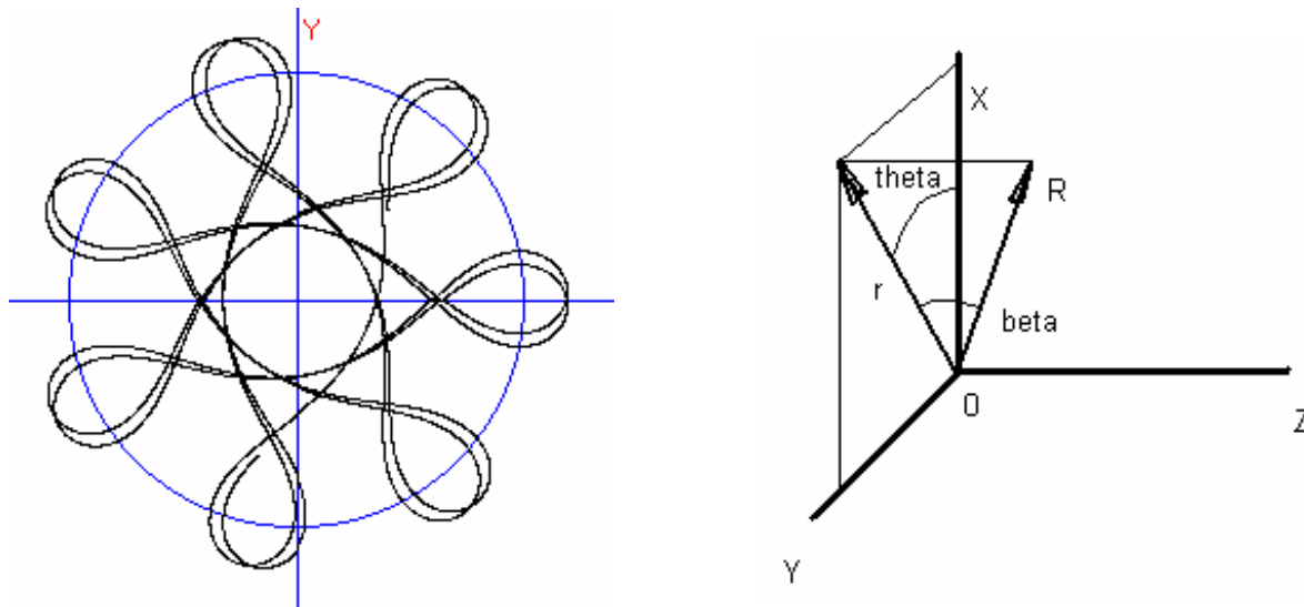
Fig.1. Protons (14.7 MeV) trajectory in X-Y plane. Typical example for particle orbits in SAE with initial parameters B=1 T, x=y=0.4 m, z=0 , \theta(\text{theta})=90^\circ , \beta(\text{beta})=0^\circ
