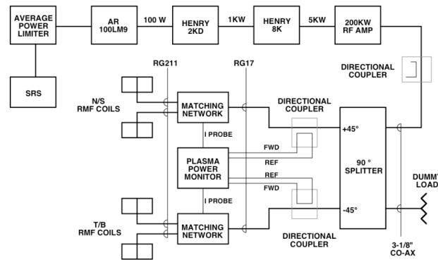
Figure 4. PFRC-2 200-kW RF system schematic.
