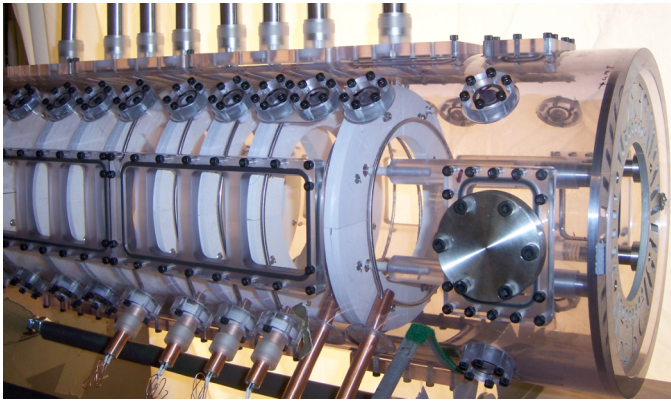
Figure 3. Photographs of the PFRC-2's polycarbonate vessel with port covers, diamagnetic loops, and BN-covered HTS FCs.
