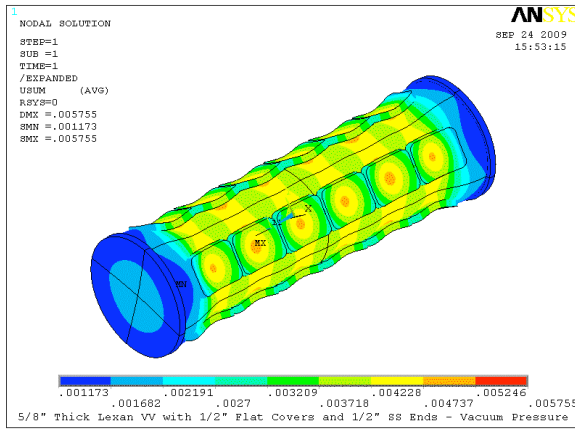
Figure 1. Calculated deflection of polycarbonate vessel, with port covers attached, under vacuum load.
