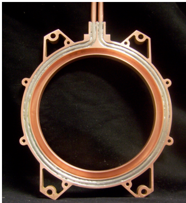
Figure 2. Copper mandrel for the outermost FC, prior to embedding the HTS. The ID is ~ 13 cm.
