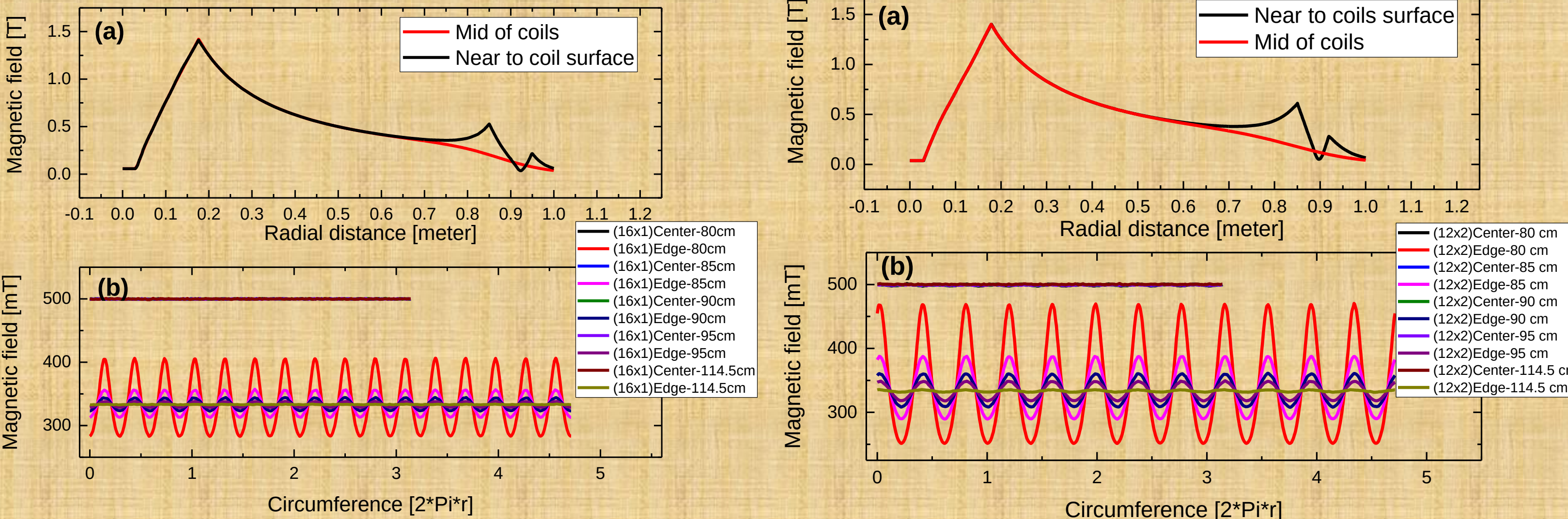
Ripple factor comparison for 16 coils (16x1) at plasma center and plasma edge for 80 cm, 85 cm, 90 cm, 95 cm and 114.5 cm of outer limbs.
