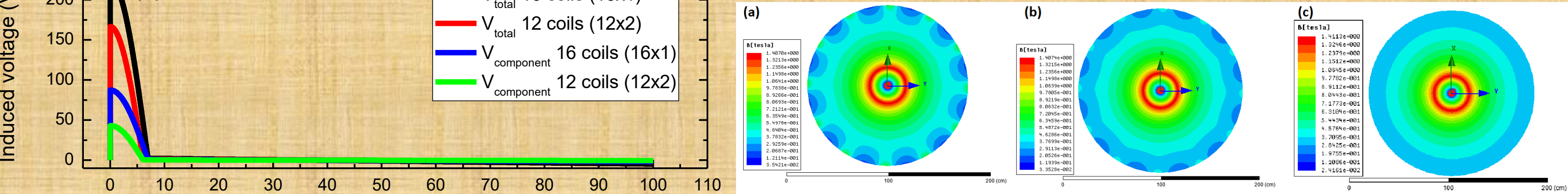
Cross sectional view of the ripple pattern of 12 coils (12x2), for 80 cm, 90 cm, and 114.5 cm radius
