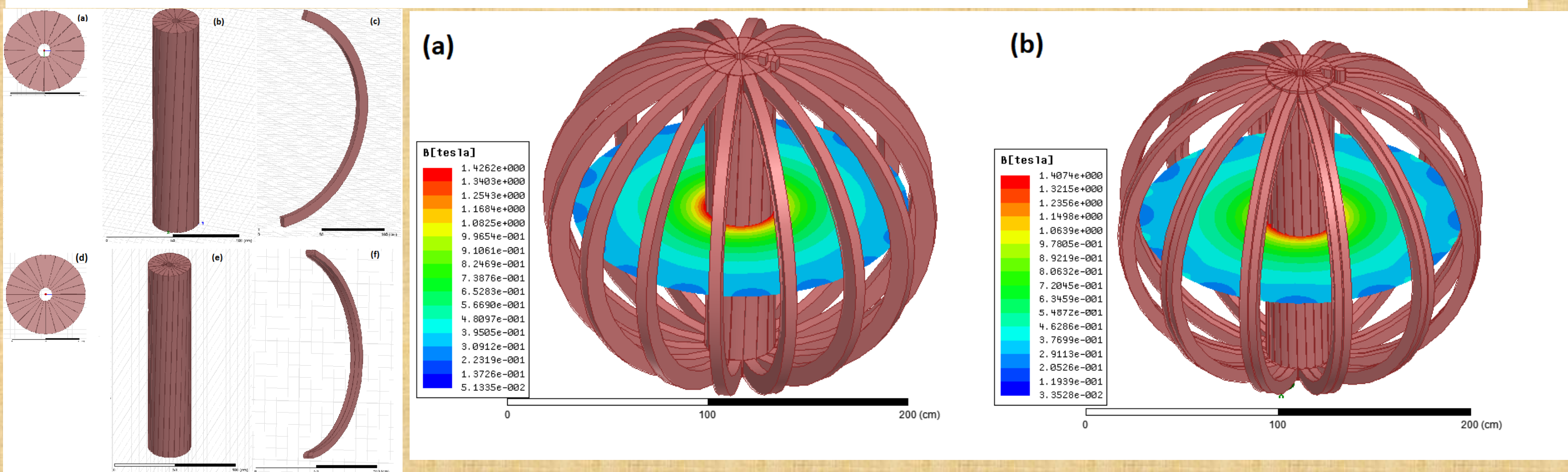
TF coils (16x1) and 12 TF coils (12x2) system. Magnetic field pattern at mid plane (a) 16 coils (16x1) and (b) 12 coils (12x2) of toroidal field coil system.
