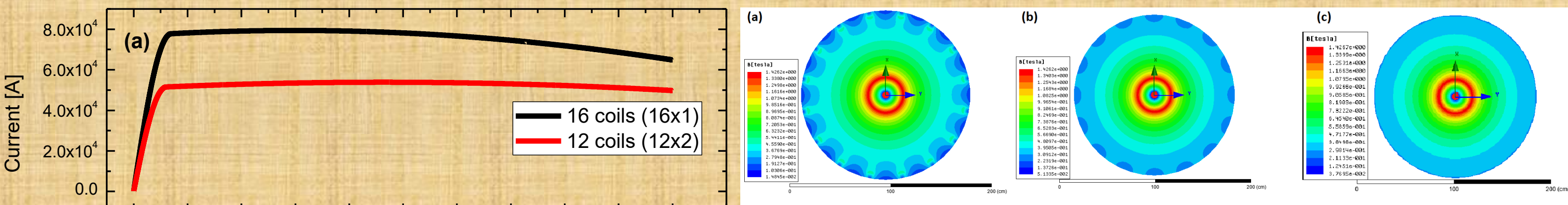
Cross sectional view of ripple pattern of 16 coils (16x1for 80 cm, 90 cm, and 114.5 cm radius .
