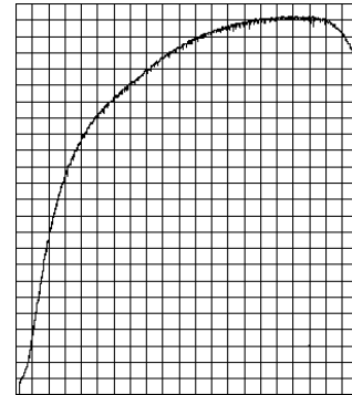
Figure 12: Stress-strain diagram for the external (superposition) demountable joint of the TF coil. Each horizontal division corresponds to a displacement of 1 mm and each vertical division to a force increment of 3.07 kN.
