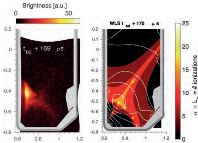
7 Visible radiation maps produced by a fast camera ( a ) compared with where Townsend modeling predicts ionization should occur ( b ). The breakdown process begins near the inner wall of TCV in contrast to where the Townsend theory model predicts it should take place: at the middle of the vessel where the poloidal magnetic field null was programmed. This is an important result for future devices which should consider in their control strategies that the breakdown may not commence at the poloidal magnetic field null.
