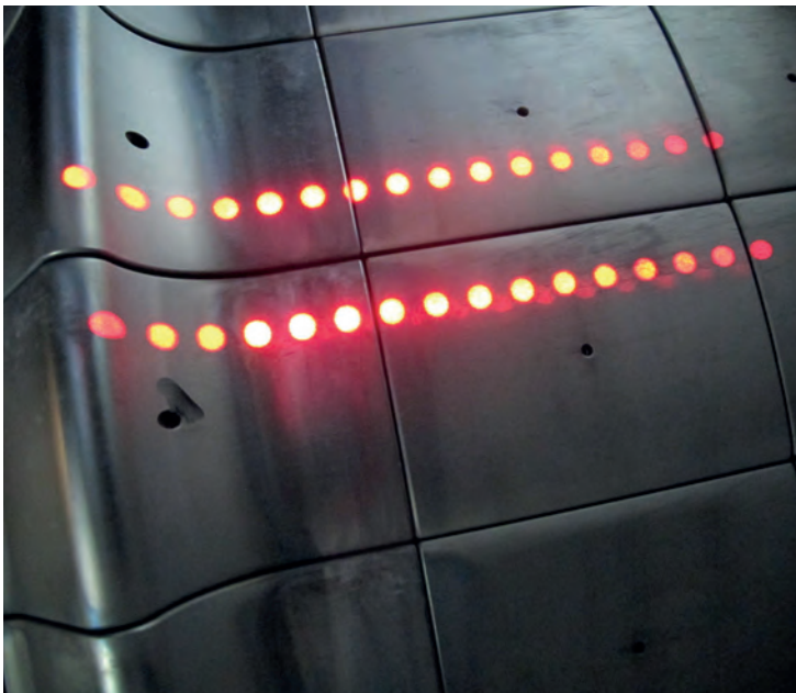
TCV Tangential DSS: in-vessel calibration.
