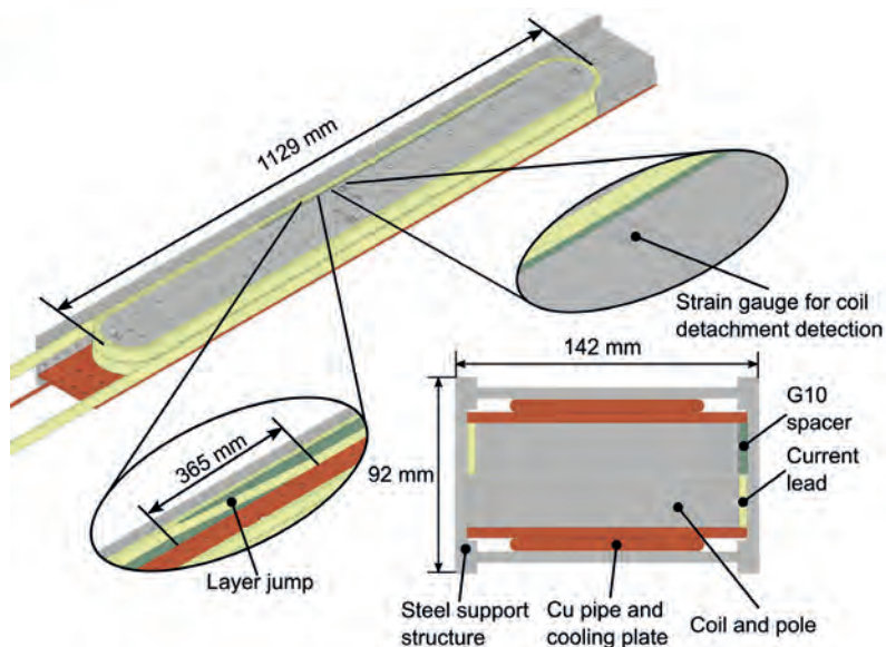
2 The EDIPO 2 subsize coil design.
