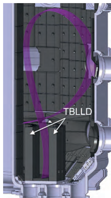
2 Initial design of the upcoming Tightly-Baffled, Long-Legged Divertor (TBLLD) in TCV.
