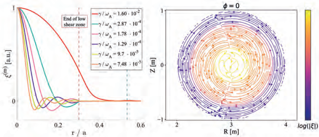
3 Spectrum of m=n=1 infernal modes, for constant q = 1.0001 in the core and q_s = 10 . Left: radial plasma displacements \xi versus minor radius, and corresponding linear growth rates \gamma/\omega_A . Right: stream plot of the displacement for the 3 rd mode in the spectrum.
