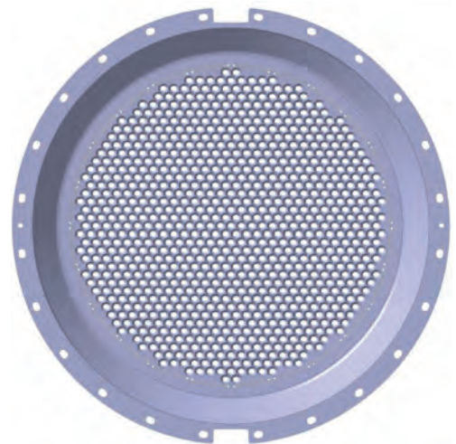
TCV DNBI: new potato-shape grid design, manufacture and tests.
