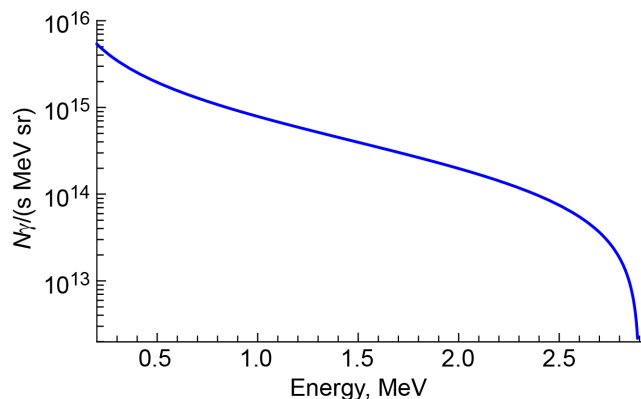
Figure 3.—Bremsstrahlung photon spectrum for electron beam end-point of 2.9 MeV, for 450- \mu A (per vial) test case (top of sample).
