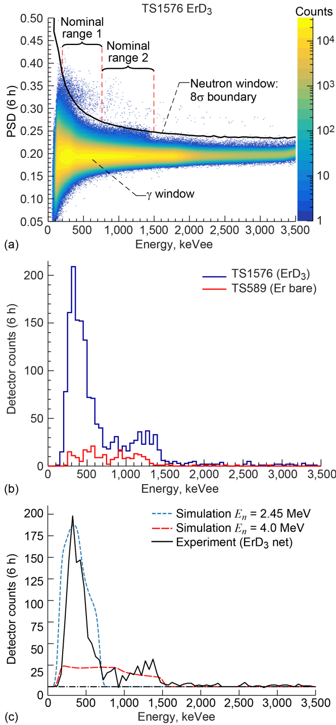
Figure 4.—Measured test data (EJ-309 HV detector) prior to unfolding (beam 2.9 MeV, 15 mA, 6 h). (a) PSD plot for TS1576 utilizing the 8 \sigma constraint window used to ensure separation of neutrons from \gamma rays. (b) Detector-measured counts for TS1576 (ErD 3 ) and TS589 (Er-bare) versus energy (50-keVee bins); (c) Comparison of measured net counts for ErD 3 with two detector simulations for a source of monochromatic neutrons with energies ( E_n ) of 2.45 MeV and 4 MeV.
