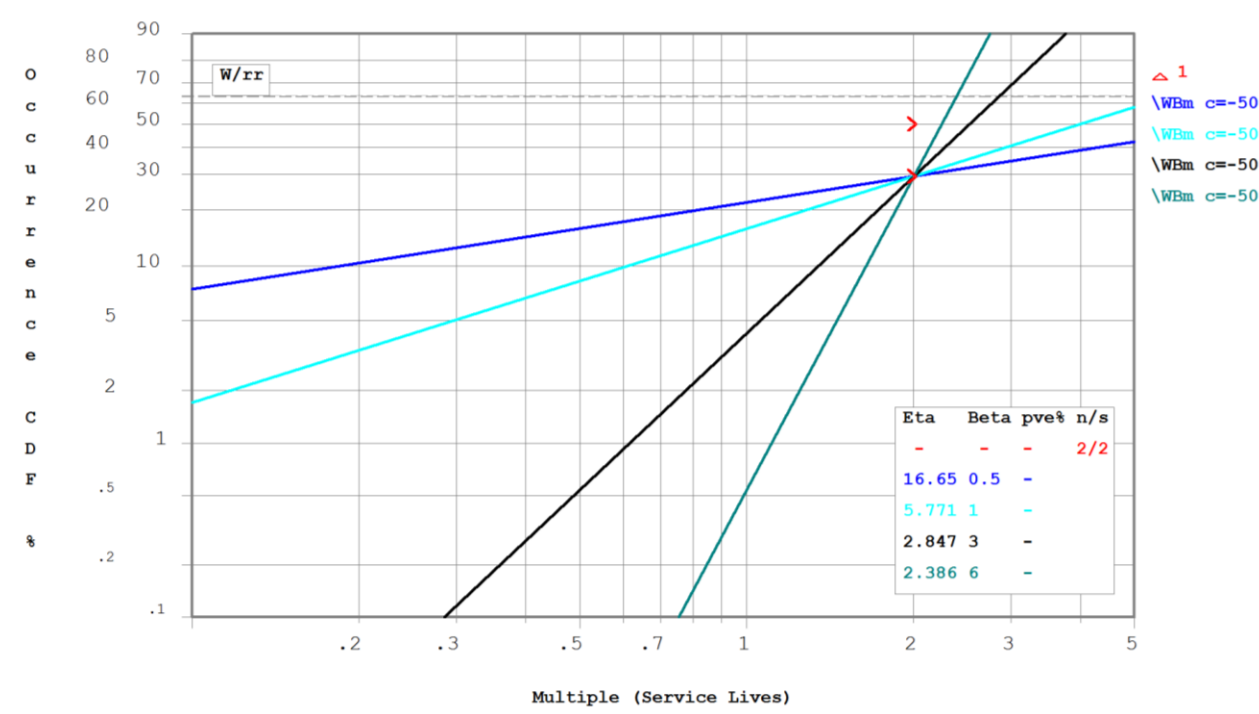
Figure A-4. Weibull analysis of a qualification program with two engine samples taken to 2 \times \text{SL} (no failures).
