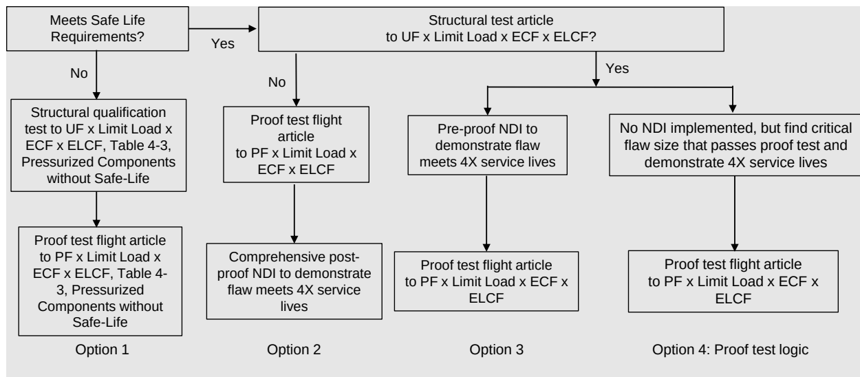
Figure 5-1. Qualification strategies for engine elements, excluding qualification by analysis (no test option) and by similarity. ECF – Environmental correction factor, ELCF – External load correction factor, UF – Ultimate Factor, PF – Proof Factor. For options relying on fracture analysis, particularly Option 4, the analysis methods should be validated by test.
