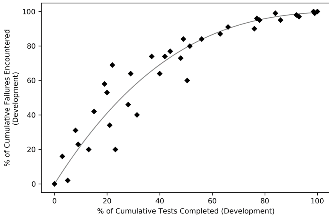
Figure 4-1. Percentage of failures encountered as a function of development test program completion for the F-1, J-2, and SSME programs (see JANNAF-GL-2012-01-R0 [19]).
