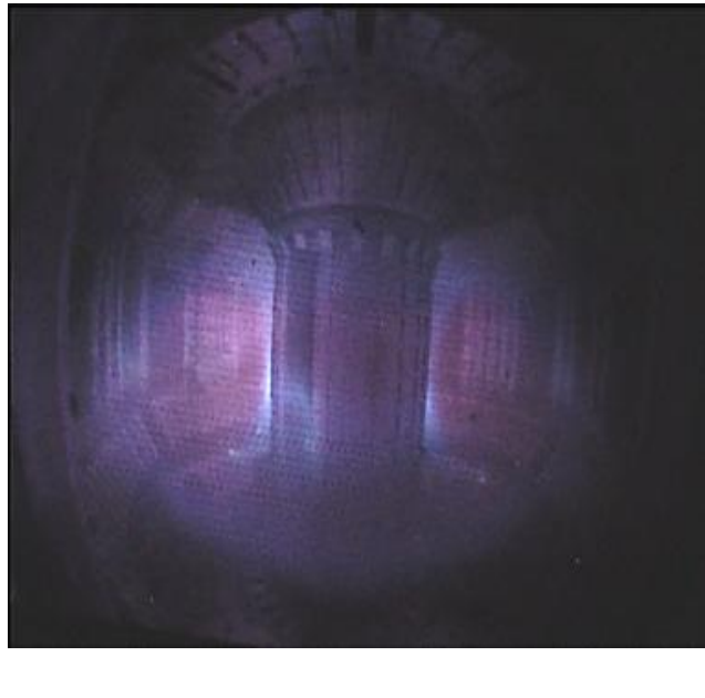
The appearance of the KTM tokamak and video frames of the plasma discharge captured by the standard color camera operated at 30 fps.
