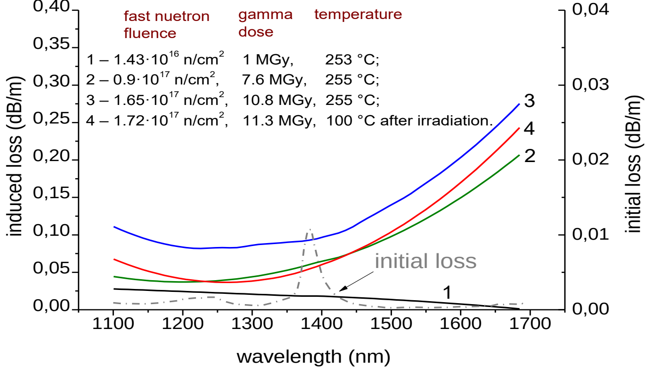
Spectrum of initial and radiation-induced optical losses in optical fibers with an undoped silica core and fluorinated cladding in a protective polyimide coating under reactor irradiation at a fast neutron flux of 2.4 \cdot 10^{13} \text{ n/cm}^2 \text{ s} and a dose rate of 1.57 \text{ kGy/s} .
