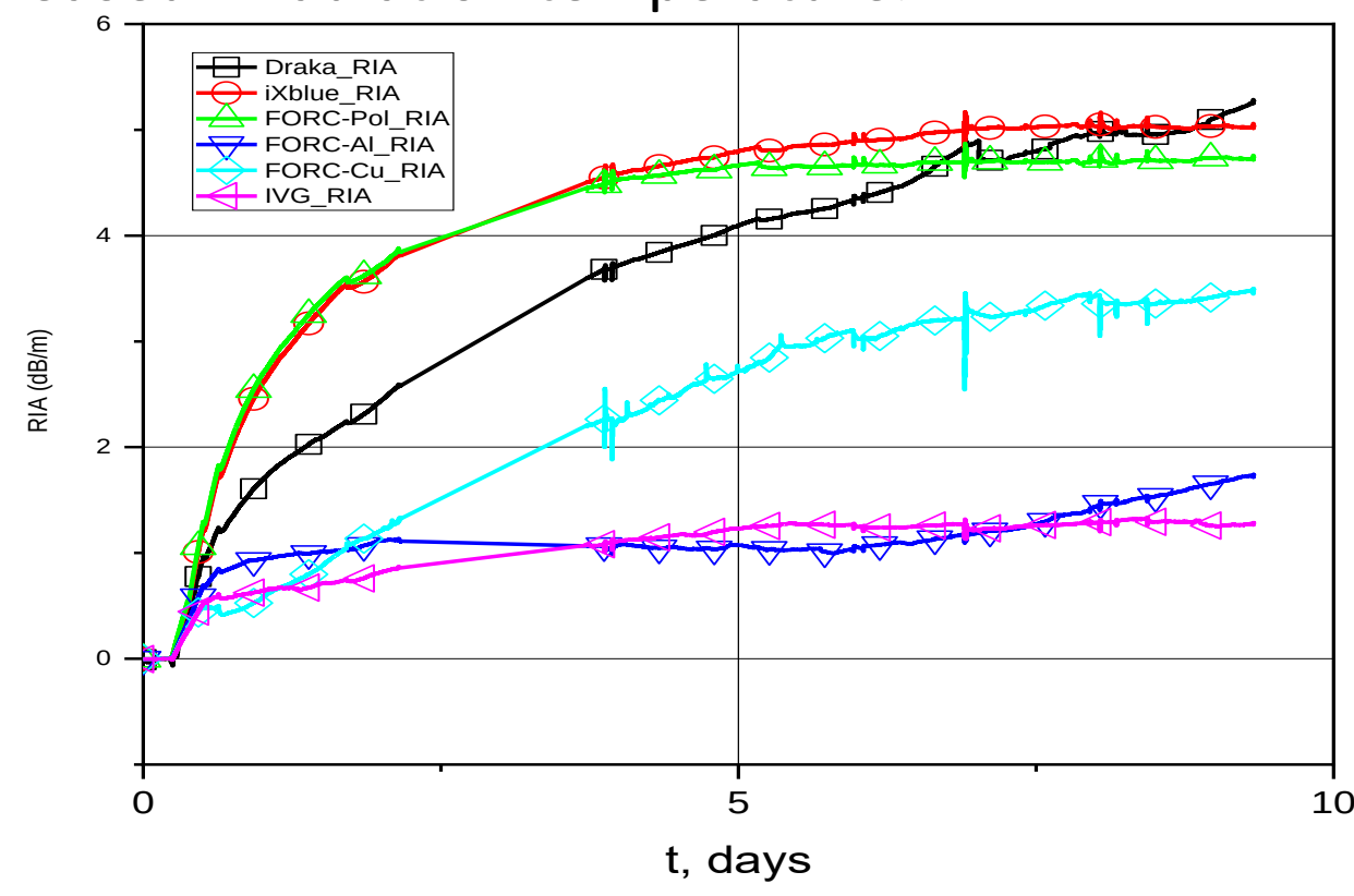
Dependence of changes in radiation-induced attenuations for different fibers on the irradiation time
