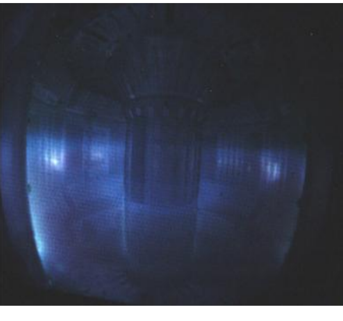
The appearance of the KTM tokamak and video frames of the plasma discharge captured by the standard color camera operated at 30 fps.
