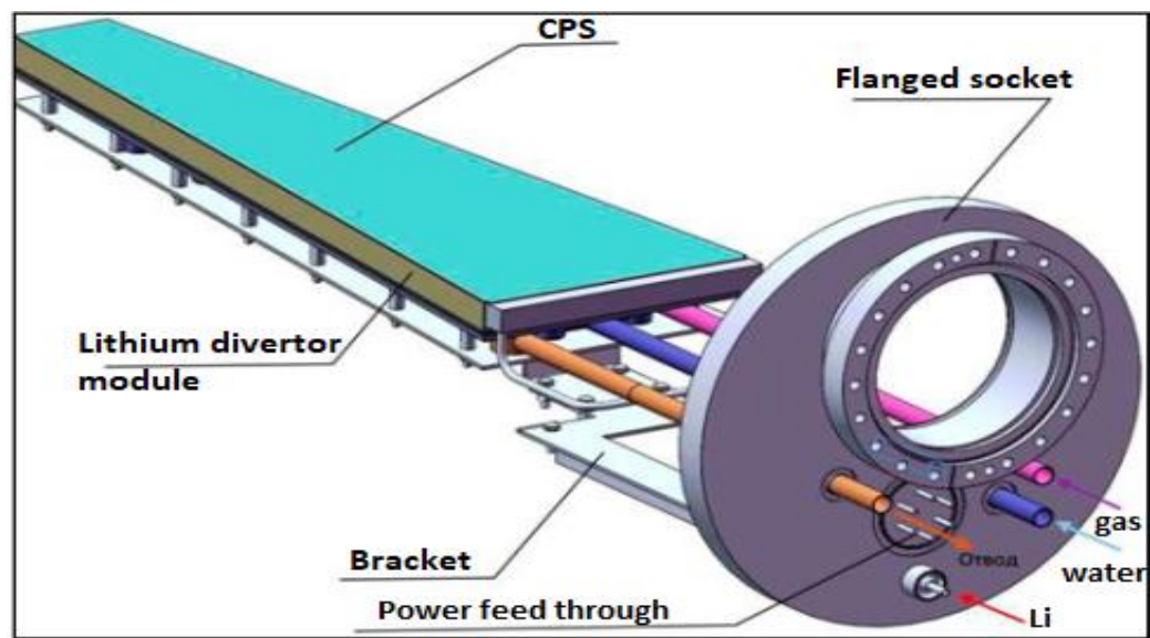
Lithium divertor module with steam-gas mixture cooling system
